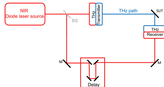
FIGURE 2. Homodyne concept for diode-laser based photonic THz systems. BS: beam splitter, SUT: sample under test, M: mirror.
