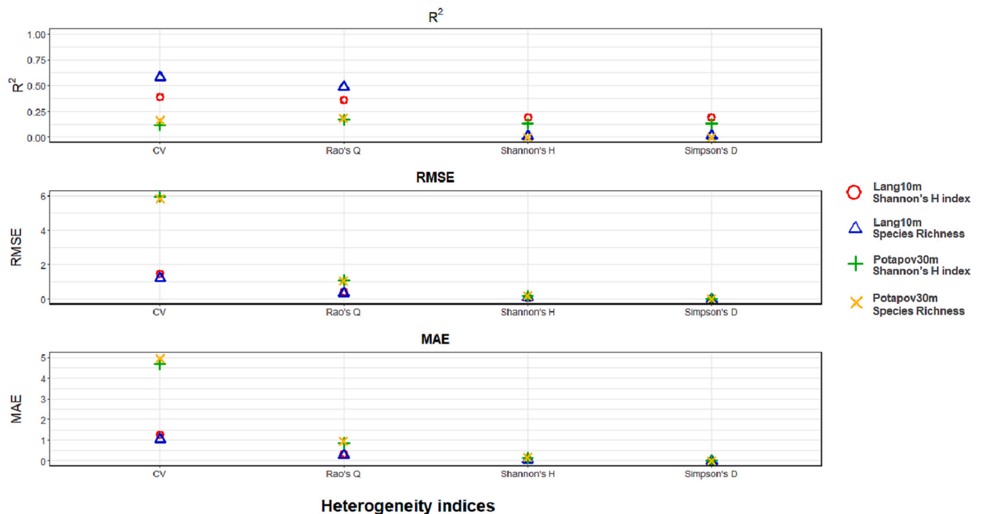
Fig. 11. R^2 , RMSE and MAE derived from the correlations between HH (calculated with the four heterogeneity indices: Rao's Q, CV, Shannon's H and Simpson's D) using the CHMs Lang10m and Potapov30m and tree species diversity (assessed through the Shannon's H index and the species richness) in the Italian study area.
