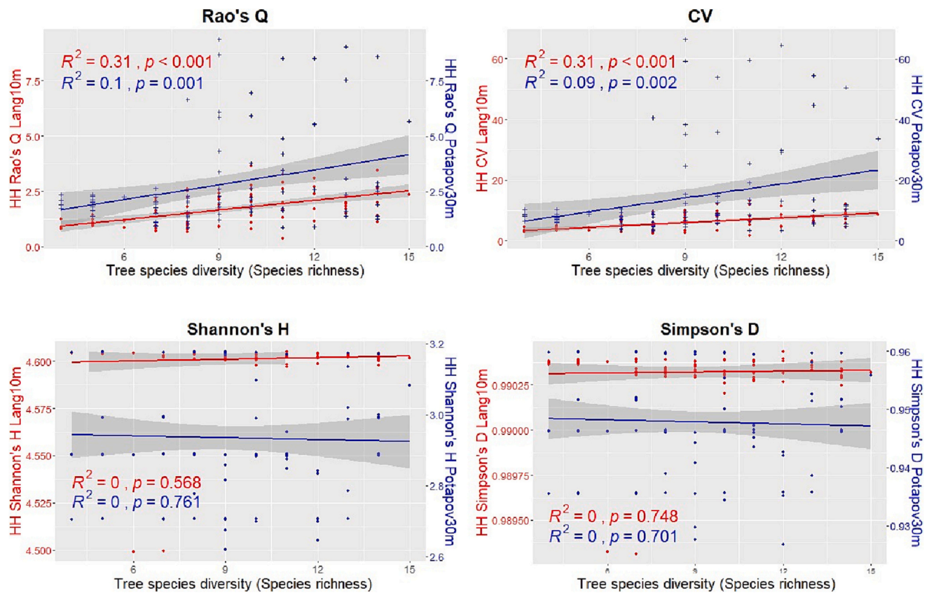
Fig. 10. Linear regressions between the tree species diversity assessed through the species richness and the HH calculated with the 4 heterogeneity indices (Rao's Q, CV, Shannon's H and Simpson's D) using both the GEDI CHMs Potapov30m (blue points and line) and Lang10m (red points and line) in the German study area.
