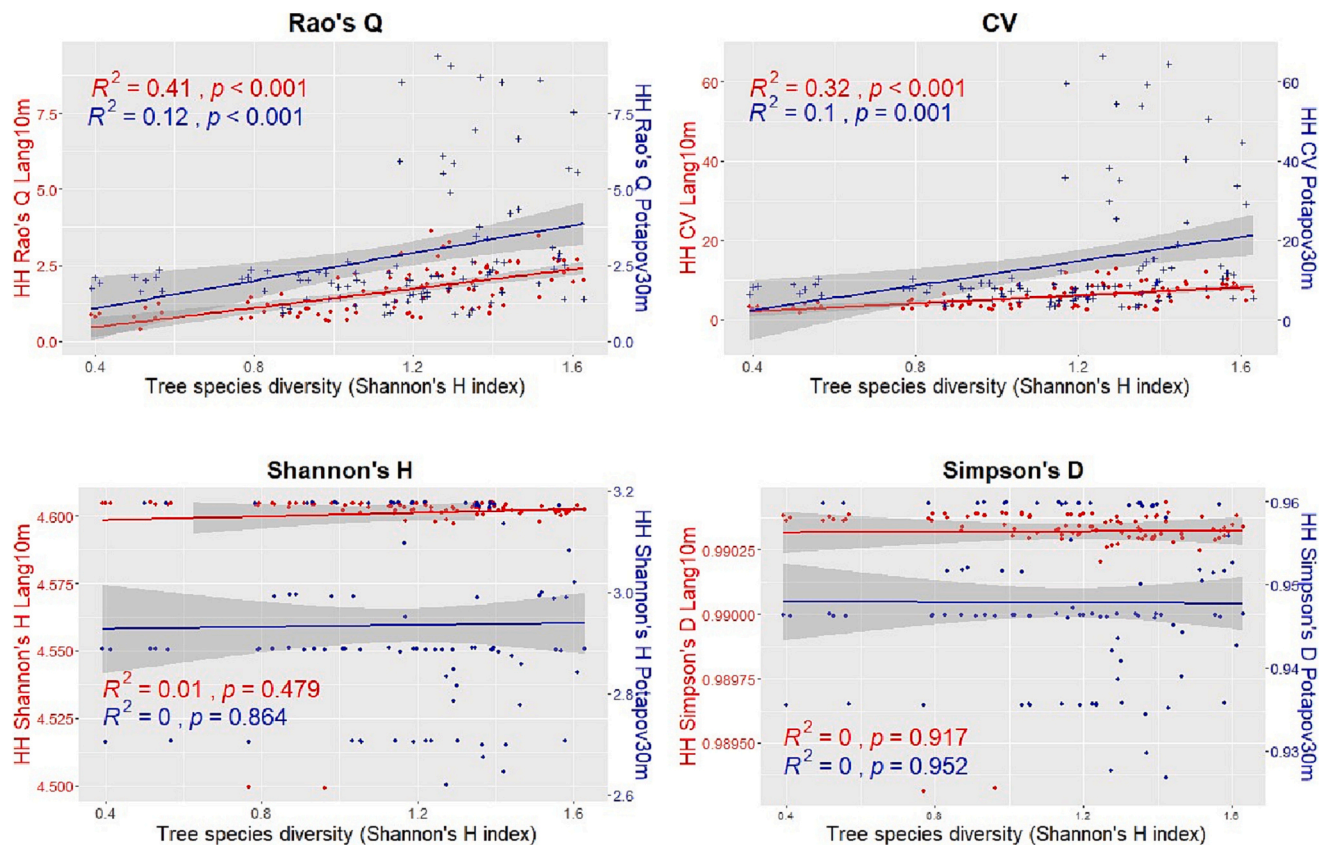
Fig. 9. Linear regressions between the tree species diversity estimated through the Shannon's H index and the HH calculated with the 4 heterogeneity indices (Rao's Q, CV, Shannon's H and Simpson's D) using both the GEDI CHMs Potapov30m (blue points and line) and Lang10m (red points and line) in the German study area. In order to better compare the results, in the sub-plots of Shannon's H and the Simpson's D, 2 different y scales have been used.
