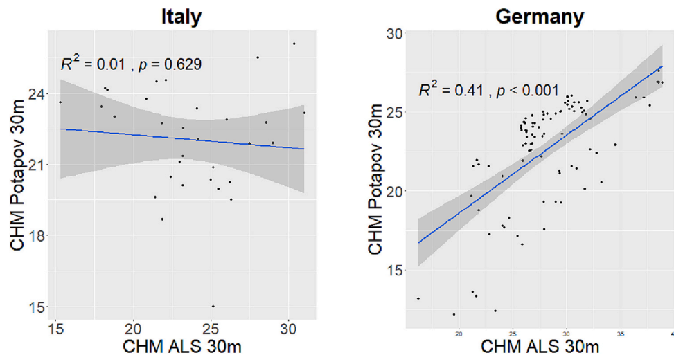
Fig. 6. Validation of the GEDI CHM Potapov30m with local ALS CHM LiDAR data at 30 m spatial resolution.
