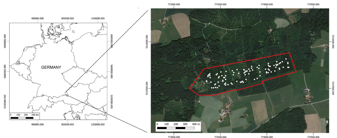
Fig. 3. The study area Traunstein (Germany). The border of the study area is shown in red. The white dots show the center of all the plots. Background image used: Google Image at February 21th 2023. Coordinates in WGS 84/ UTM zone 32 N (EPSG:32632).
