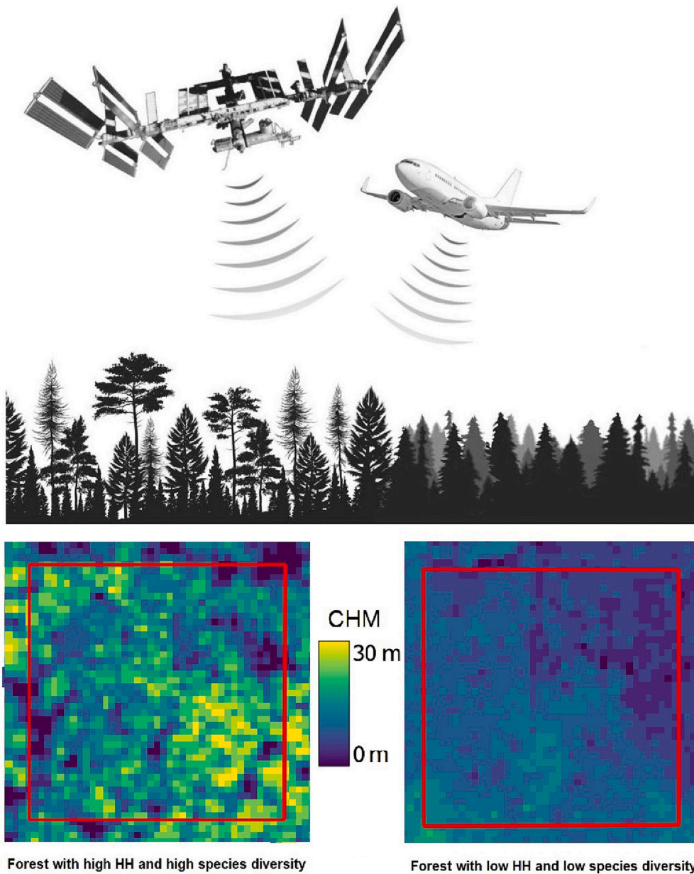
Fig. 1. The figure summarizes the aim of our study. Forests with high HH (assessed through CHM LiDAR data) have a complex vertical structure (seen from the side in the upper figure and from above in the lower figure), high environmental heterogeneity and high tree species diversity (forest on the left). On the other hand, forest with low HH might have lower species diversity (forest on the right). This concept has been already tested measuring the HH with airborne LiDAR data. In this study we test it using the recently published and freely available LiDAR GEDI CHMs Lang10m and Potapov30m.
