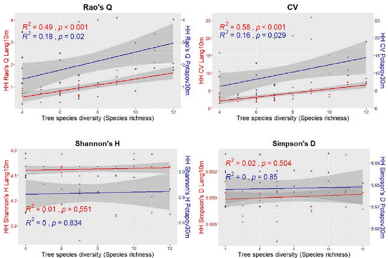
Fig. 8. Linear regressions between the tree species diversity assessed through the species richness and the HH calculated with the 4 heterogeneity indices (Rao's Q, CV, Shannon's H and Simpson's D) using both the GEDI CHMs Potapov30m (blue points and line) and Lang10m (red points and line) in the Italian study area. In order to better compare the results, in the sub-plots of Shannon's H and the Simpson's D, 2 different y scales have been used.
