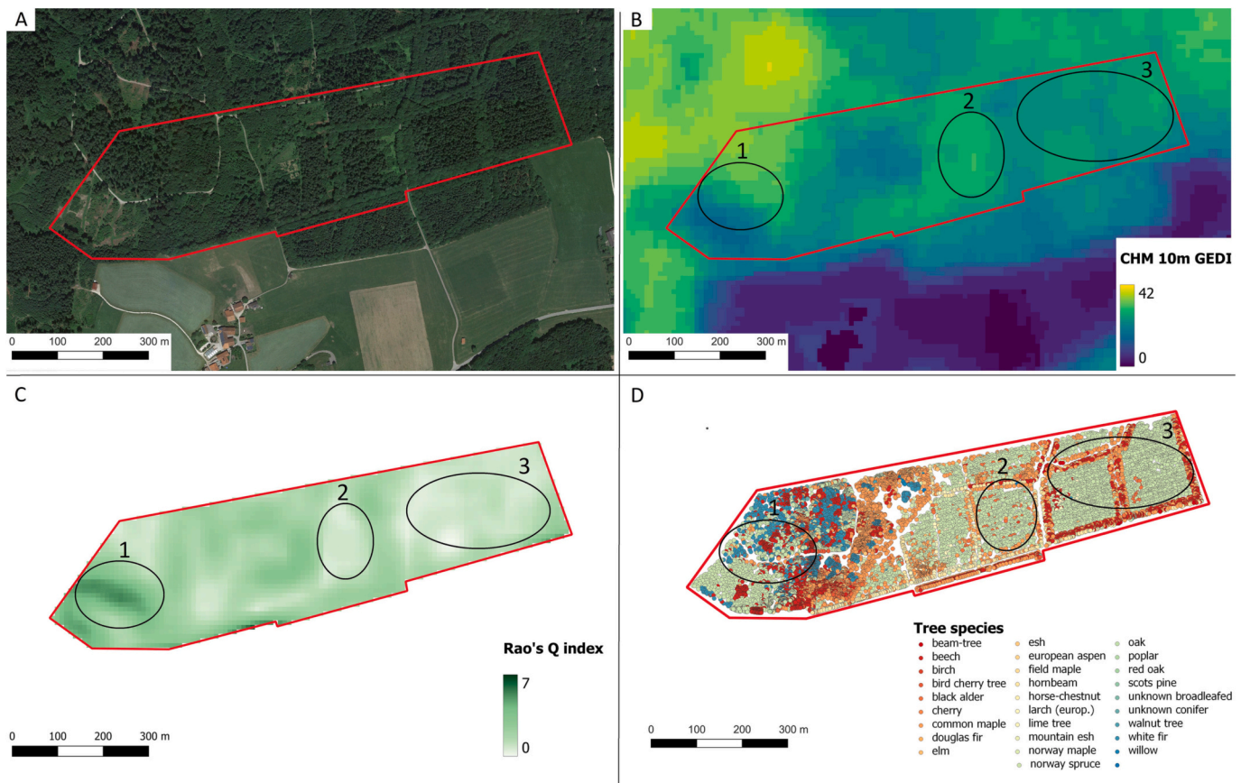
Fig. 14. Sub-figure A shows the RGB image of the Traunstein area (Google Image June 15th 2021). Sub-figure B shows the GEDI CHM Lang10m. Sub-figure C shows the Rao's Q values for the whole area while sub-figure D the tree species location. The circle 1 shows as an example a forested area with heterogeneous tree height (heterogeneous colours/heights in sub-figure B) with higher Rao's Q values (dark green values in sub-figure C) and with high tree species diversity (sub-figure D). On the other hand, black circle 2 and 3 show areas with homogeneous tree height (homogeneous colours/heights in sub-figure B), low Rao's Q values (lighter green values in sub-figure C) and low tree species richness (sub-figure D).
