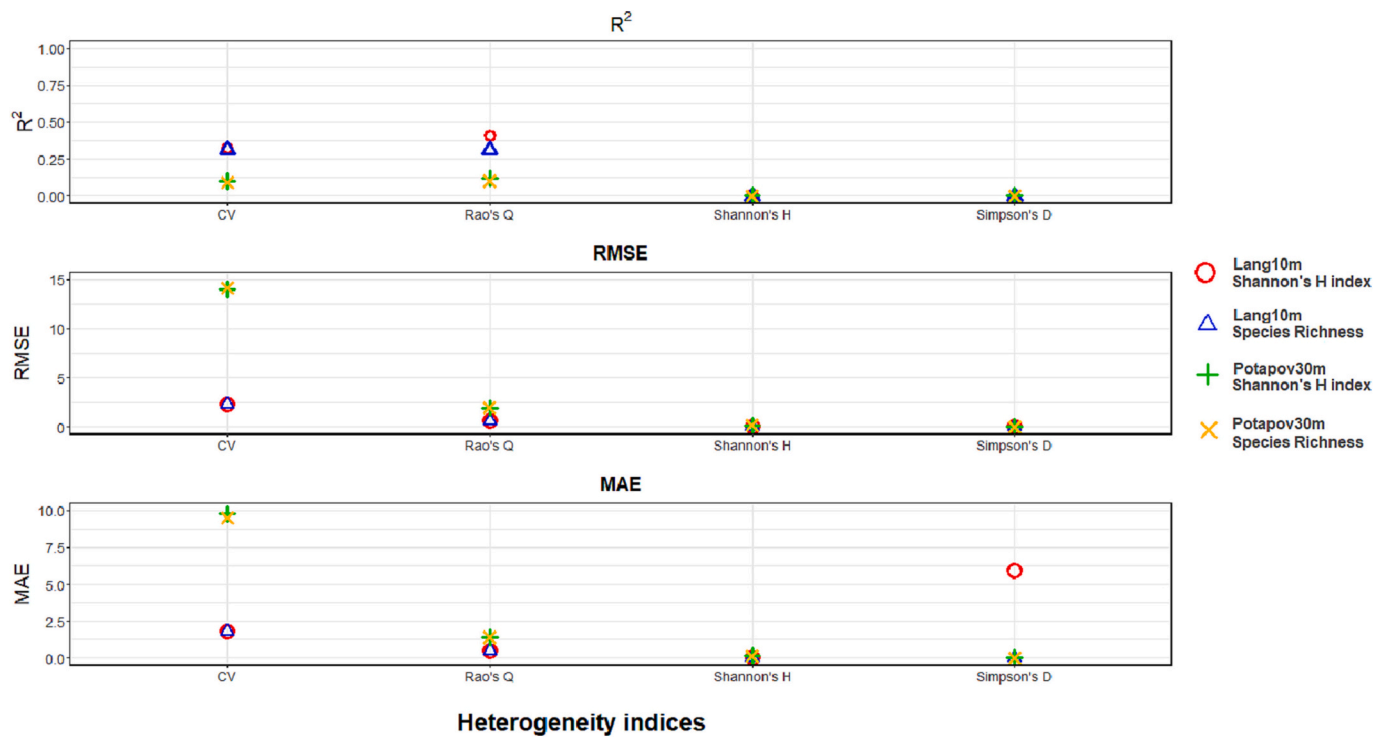
Fig. 12. R^2 , RMSE and MAE of the correlations between HH (calculated with the four heterogeneity indices: Rao's Q, CV, Shannon's H and Simpson's D using the CHMs Lang10m and Potapov30m) and tree species diversity (assessed through the Shannon's H index and the species richness) in the German study area.
