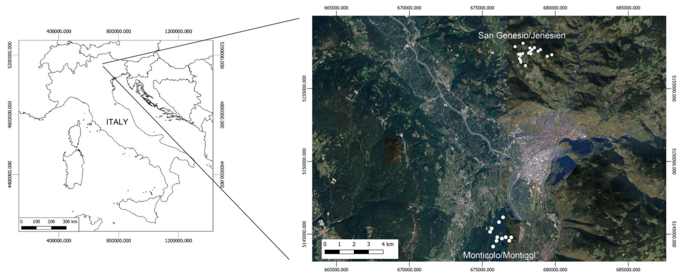
Fig. 2. In white, the center of the 30 plots situated in the 2 forested areas of San Genesio/Jenesien and Monticolo/Montiggel in South Tyrol (Italy). Background image used: Google Image at February 21th 2023. Coordinates in WGS 84/ UTM zone 32 N (EPSG:32632).
