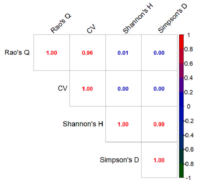
Fig. 13. Correlation matrix ( R^2 ) between the HH calculated with the four heterogeneity indices (Rao's Q, CV, Shannon's H and Simpson's D). The data refers to the results of Table 3.
