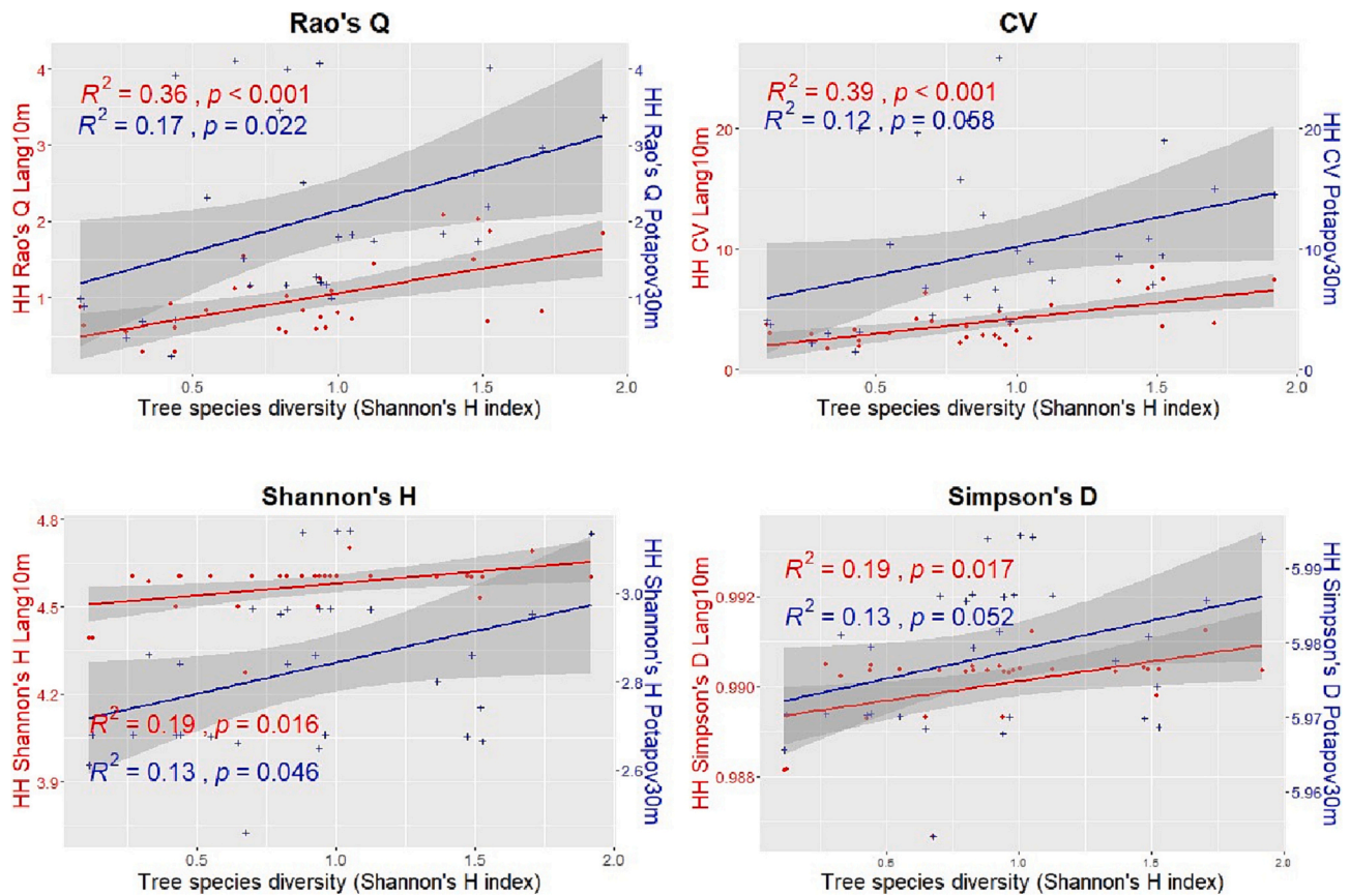
Fig. 7. Linear regressions between the tree species diversity estimated through the Shannon's H index and the HH calculated with the 4 heterogeneity indices (Rao's Q, CV, Shannon's H and Simpson's D) using both the GEDI CHMs Potapov30m (blue points and line) and Lang10m (red points and line) in the Italian study area. In order to better compare the results, in the sub-plots of Shannon's H and the Simpson's D, 2 different y scales have been used.
