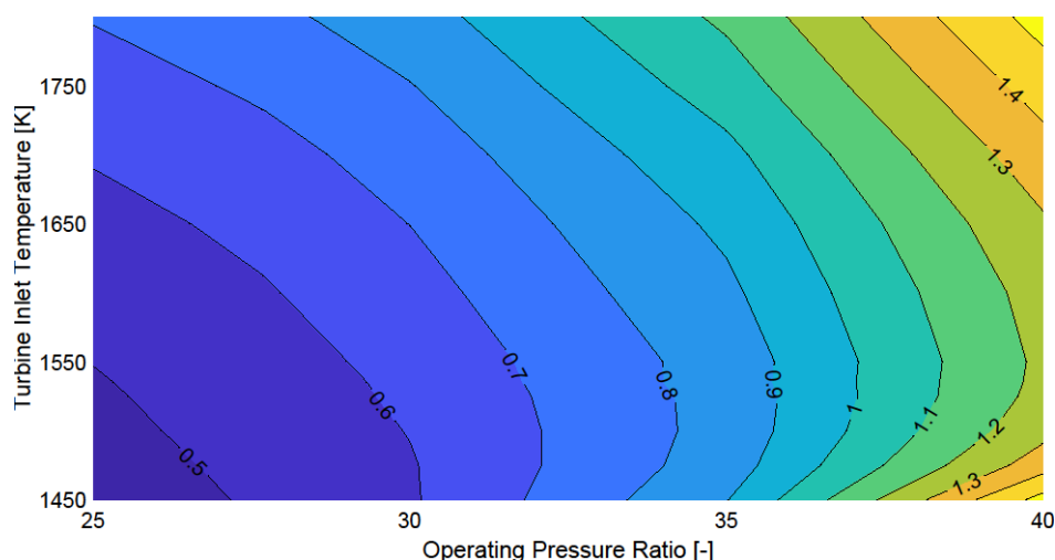
Figure 15. Cruise \text{NO}_x emissions of the fleet with varying OPR and TIT for the TAPS-II combustor configurations, normalized to the baseline, which is 3.11 t( \text{NO}_2 ) (Table 1).
