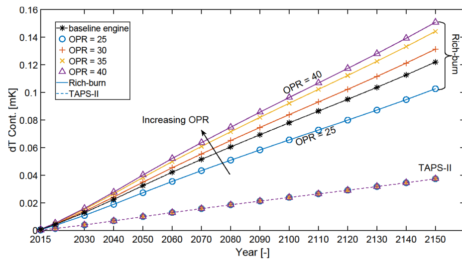
Figure 20. Temporal evolution of the temperature response due to contrail effects ( dT_{\text{Cont.}} ) for baseline engine (dotted asterisk line) and the OPR range from 25 to 40. Solid lines represent rich-burn configurations, whereas dashed lines represent TAPS-II configurations.
