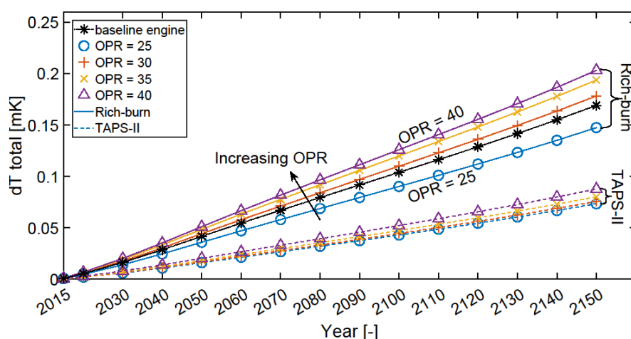
Figure 22. Temporal evolution of the total temperature response for baseline engine (dashed asterisk line) and an OPR ranging from 25 to 40. Solid lines represent rich-burn configurations, whereas dashed lines represent TAPS-II configurations.
