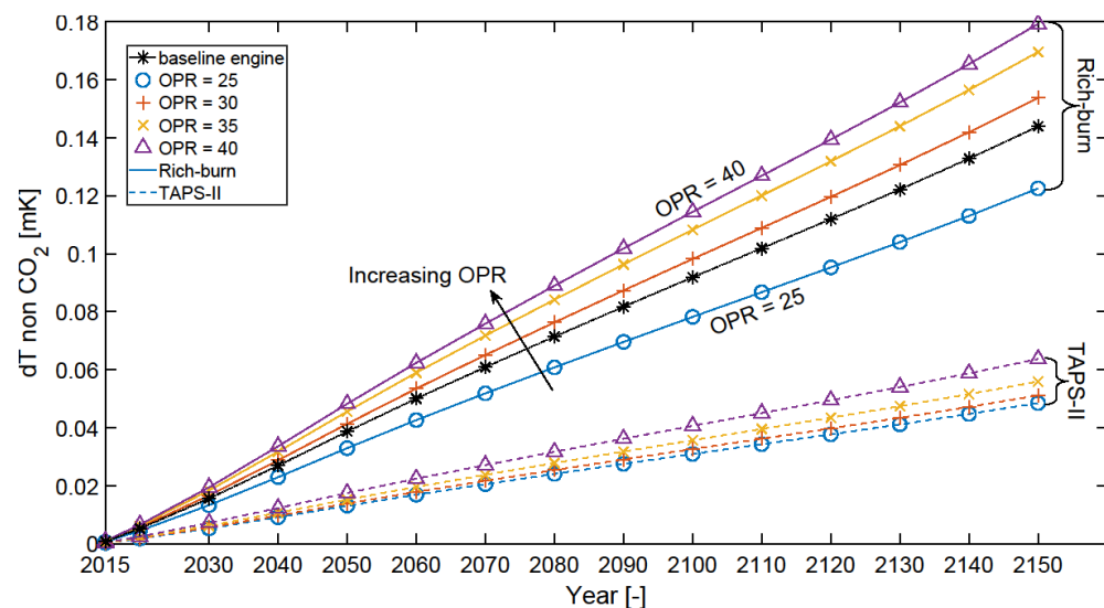
Figure 21. Temporal evolution of the temperature response due to the non- \text{CO}_2 emissions ( dT_{\text{NO}_x} , \text{H}_2\text{O} , and contrails) for baseline engine (dotted-asterisk line) and the OPR range from 25 to 40. Solid lines represent rich-burn configurations, whereas dashed lines represent TAPS-II configurations.
