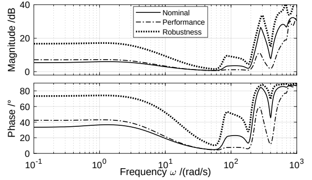
FIG 20. Multiloop output disk margins for different cases
