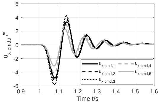
FIG 15. Commanded control surfaces for H = 3\text{m}
