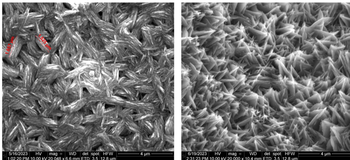
Figure 2. E-SEM images magnesium deposition at 1 mA cm -2 for 42 min from Mg[B(HFIP) 4 ] 2 /DME (left), and Mg[B(HFIP) 4 ] 2 /MgCl 2 /DME (right) electrolyte solutions.
