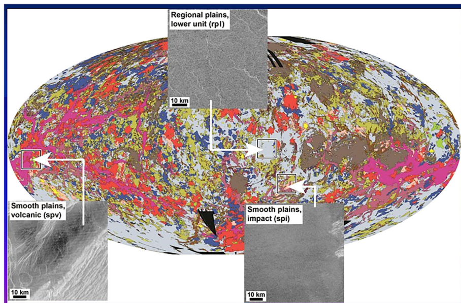
Fig. 23 Potential landing sites for the Venera-D Lander
