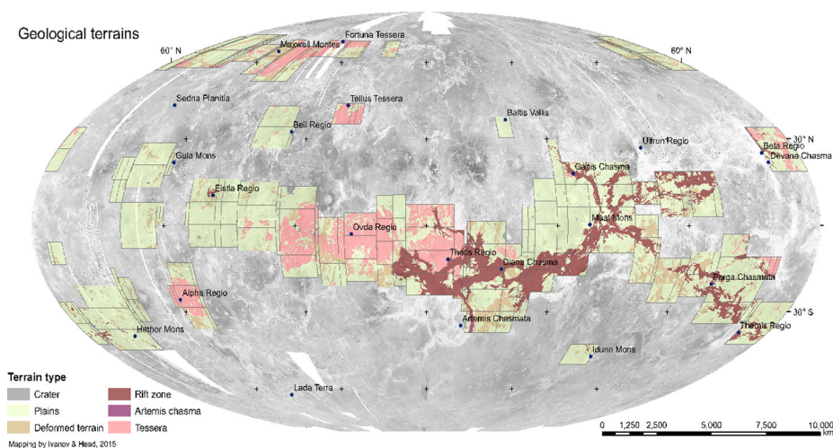
Fig. 15 Map of geological terrains and named landmarks covered by the Regions of Interest (RoIs) defined in EnVision's Science Operations Reference Scenario. The RoIs are chosen to include representative samples of all major geological terrain and feature types. These different features are not distributed at random but are in specific, known locations. EnVision's approach is to define roughly thousand-kilometer square RoIs covering most of the highlands and a representative selection of the lowland features. This strategy allows to progressively build up along the 6 cycles the required global and targeted measurements dataset, in particular over all pre-selected regions of interest, which represent a fraction of about 30% of Venus surface. Definitions of geological terrain types are as mapped by Ivanov and Head (2015)
