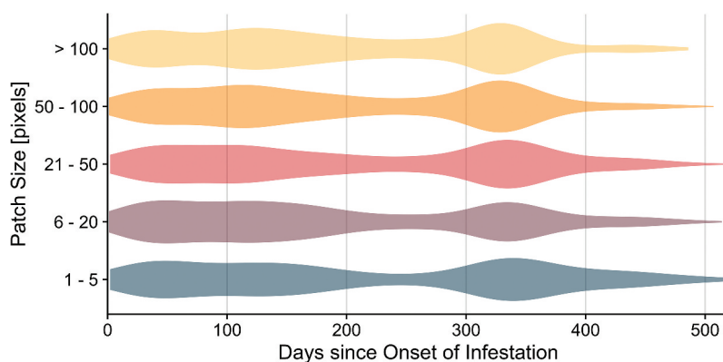
Figure 12. Distribution of values regarding the timeliness of detection in patches of different sizes for the years 2016–2019, as determined using Sentinel-2 random forest configuration
