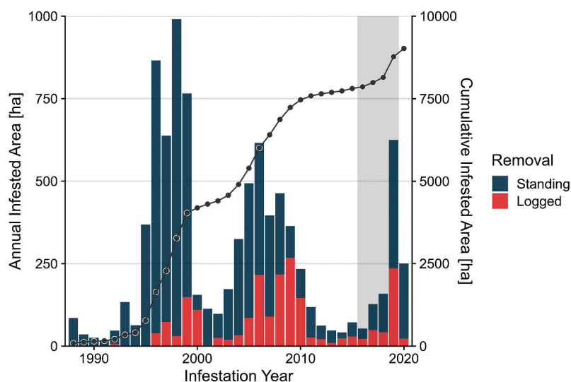
Figure 2. Time series of area infested by bark beetles in the BFNPP. Columns represent yearly increase in infested areas, and lines/dots the cumulative infested area. The study period is marked by the grey box. Infested areas that have been left standing, which were used in this study, are colored in blue.
