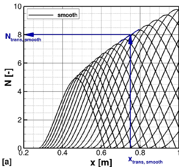
Fig. 7 Transition prediction using e^N -method, Re_m = 4.0 \times 10^6/m
