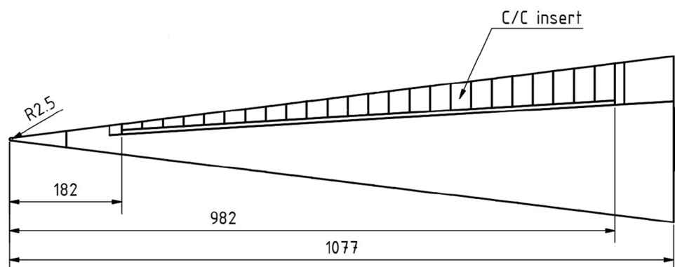
Fig. 2 HEG wind tunnel model with exemplary C/C insert. All dimensions are provided in millimeter
