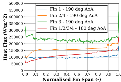
Figure 12: Comparison of fin leading edge heat flux for 180 and 190 degree AoA cases
