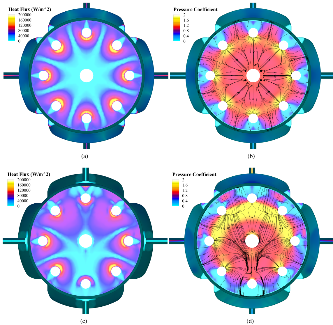
Figure 13: Images from start of glide for (a) baseplate heatflux at 180 degree AoA, (b) baseplate pressure coefficient at 180 degree AoA, (c) baseplate heatflux at 190 degree AoA and (d) baseplate pressure coefficient at 190 degree AoA
