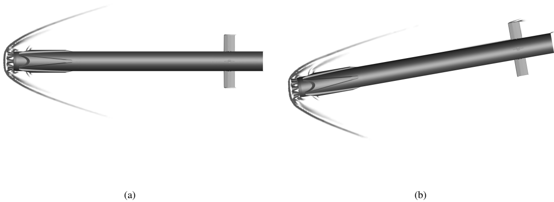
Figure 11: Symmetry plane density gradient magnitude for (a) 180 degree AoA and (b) 190 degree AoA
