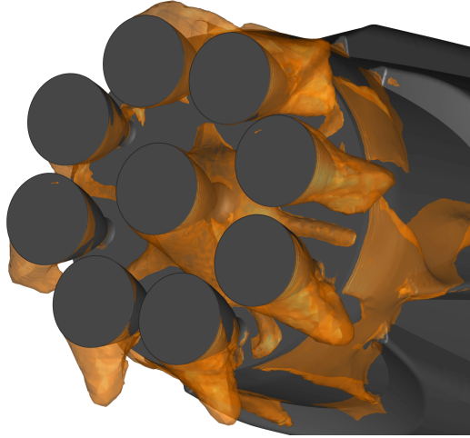
Figure 14: Isosurface showing regions of reversed flow for the 190 degrees AoA case
