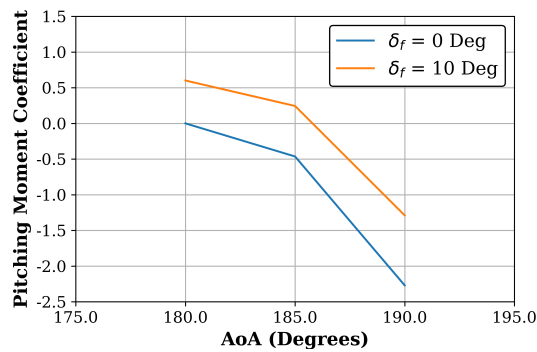
Figure 15: Pitching moment vs AoA for fin deflections of 0 and 10 degrees
