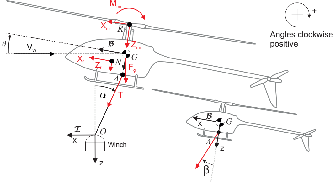
Fig. 2 Forces and moments acting on the helicopter.
