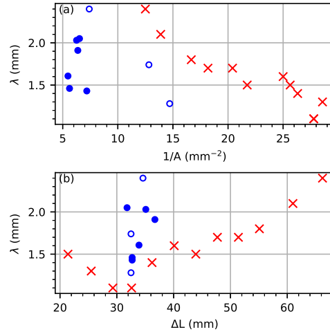
FIG. 6. Dependence of the measured wavelength \lambda on (top) the inverse of the area A of the Voronoi cells, which is proportional to the microparticle number density, and (bottom) the electrode distance \Delta L for the flight experiments a) (blue empty) and b) (blue filled circles), and the ground experiment (red crosses). Error bars for the ground data are of the size of the plot symbols (the uncertainty of \lambda is defined by the shift of the slab in the correlation analysis by 1 px = 0.0765 mm). For the flight experiments (blue symbols), both the minimum and maximum wavelengths given in Table I are represented by separate circles.
