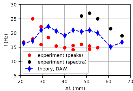
FIG. 11. Comparison of the measured wave frequencies (red circles: frequency peaks, black circles: broader spectra) with frequencies corresponding to the standard dust acoustic wave (diamonds) at different plasma compressions.
