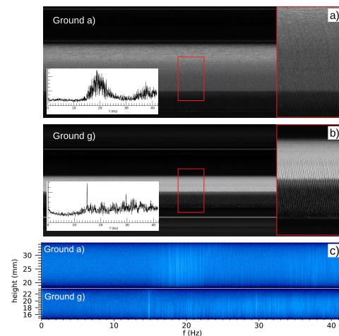
FIG. 5. a,b) Periodograms of data sets 'ground a)', 'ground g)'. The insets on the right enlarge a region to make the wave structure more visible. c) Spectra obtained by Fourier transforming the periodograms along the time domain for the ground experiments a) (top) and g) (bottom). The vertical axes show the position above the bottom electrode. The respective vertically summed-up spectra are shown as insets on the left in Figs. a) and b).
