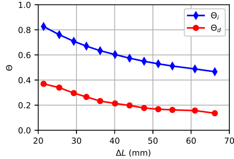
FIG. 9. Variations of the collisionality parameters for ions \theta_i = \nu_{in}/\omega_{pi} and particles \theta_d = \nu_{dn}/\omega_{pd} , versus the electrode separation \Delta L [mm]. Calculation are done for the case M_i \lesssim 1 .
