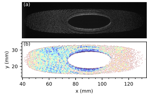
FIG. 1. a) Image of a dusty plasma under "microgravity" conditions, showing the typical "void" structure as well as concentric crests of a self-excited dust wave. The image corresponds to the instant of time between regions I and II shown in the periodogram in Fig. 3 a). b) Detected particle positions color-coded by the area of the surrounding Voronoi cells varying between 0.05 mm 2 or smaller (black) and 0.25 mm 2 or larger (red). The vertical position y is given in mm above the bottom electrode.
