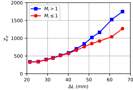
FIG. 7. Charge number Z_d as a function of electrode separation \Delta L [mm] for particle radius: a = 0.65 \mu\text{m} calculated for the plasma and particle parameters near the upper ( M_i \lesssim 1 ) and lower ( M_i > 1 ) boundary of the region where the waves were excited.
