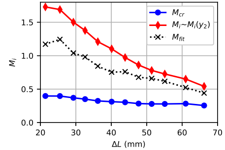
FIG. 8. Ion Mach number M_{cr} (blue dots) corresponding to the critical field, Eq. (1), and ion Mach number M_i \sim M_i(y_2) (red diamonds) following from the electric field providing the balance of the electric and gravitational forces (close to numerical estimations of E(y_2) ) as a function of the distance between the electrodes in the ground experiments. Also shown is the ion Mach number M_{fit} (black crosses) obtained from a fit of the theoretical model to the experimentally obtained wave numbers, as described in the text below.
