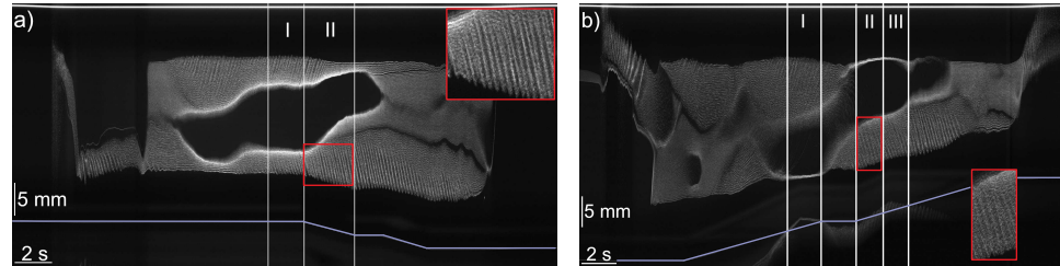
FIG. 3. Space-time plots (periodgrams) of the particle clouds during two parabolas, denoted Flight aI-II (a) and bI-III (b) in Table I. The periodgrams are produced by summing up the central 8.3 mm wide region of each original image in the time sequence in horizontal direction and stacking all resulting line plots next to each other. In these images, the pixel brightness is proportional to the particle number density 22 . Here, the direction of gravity before and after the parabolas is up due to the orientation of the cameras. The central void can be seen as empty region in the middle of the images. Wave crests are visible as diagonal bright stripes. The Roman numerals I – III mark the analyzed regions. The blue solid lines indicate the position of the moving electrode (the other electrode was held fixed at the position of the horizontal solid white line visible in the top of the images). Note that in Fig. 3b) the reflections of particles in the lower image part are reflections off the guard ring, not the electrode.
