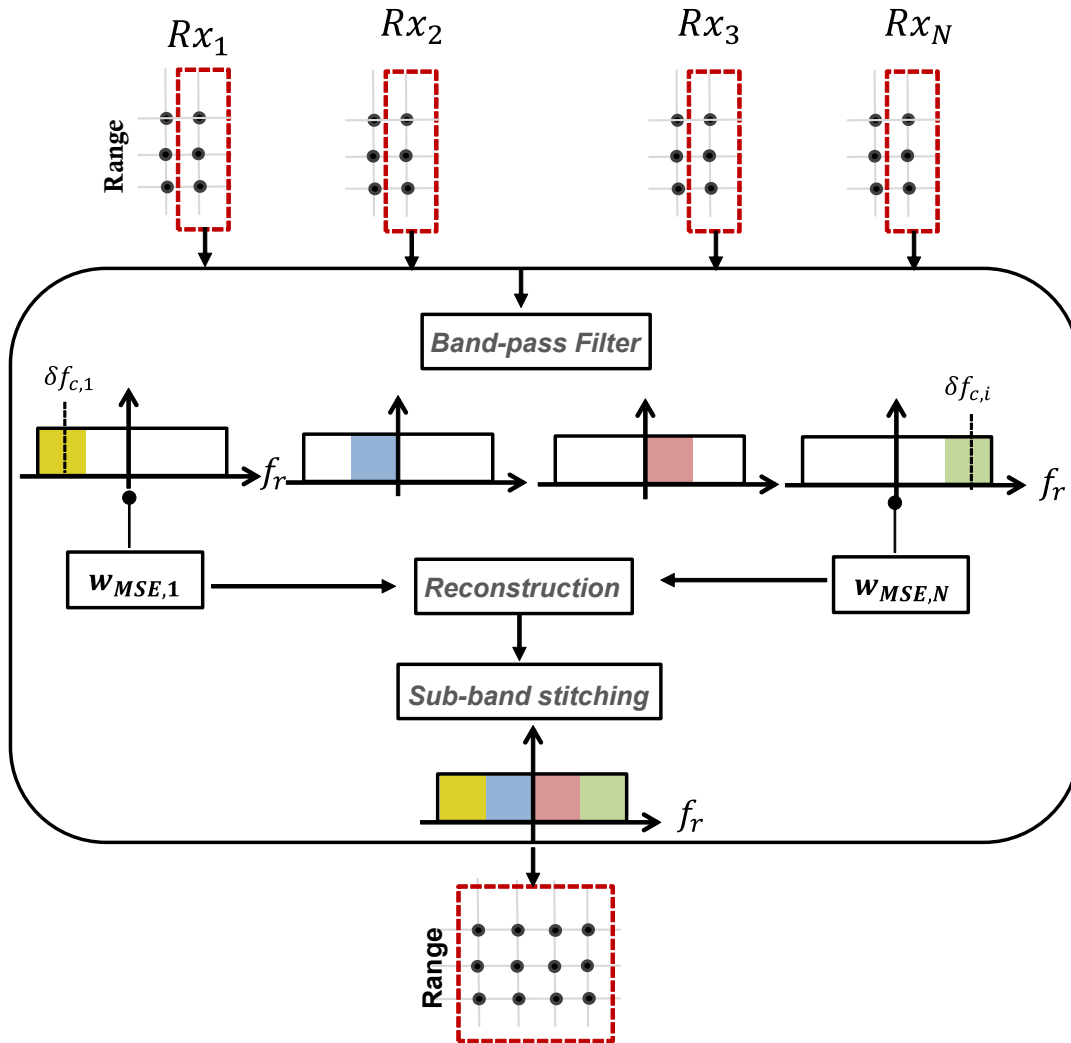
FIGURE 4.15: Band-pass filter approach: Illustration of polychromatic time-domain reconstruction. The input data are filtered in the range-frequency domain and brought back to the time domain for the reconstruction with the center frequency of each sub-band. After the simultaneous reconstructions, the sub-bands are stitched in range-frequency domain and the initial range sampling is retrieved.
