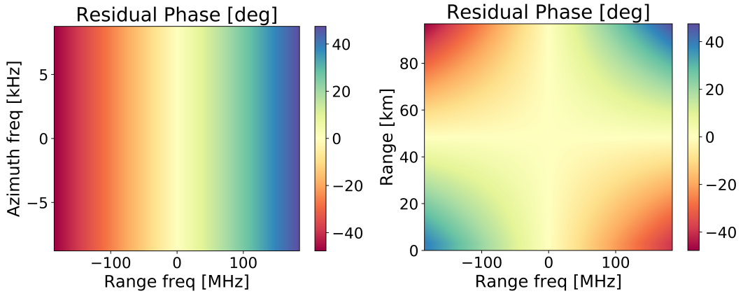
FIGURE 4.5: Residual phase after removal of the monochromatic part of Eq. (4.3) for the simulation scenario of Figure 4.11 (left) in the wavenumber domain for a near range target and (right) in the range-range frequency domain for f_a = 0 .
