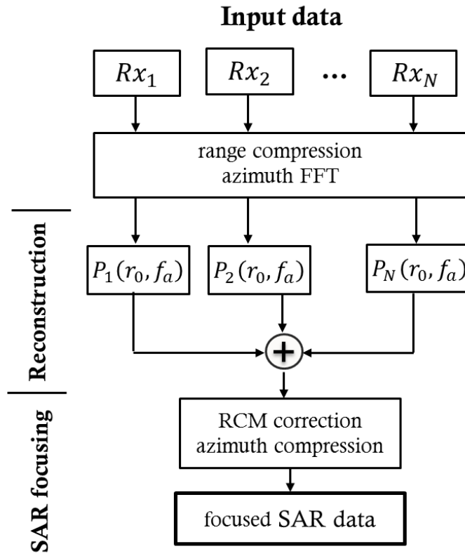
FIGURE 3.3: Block diagram of conventional Doppler-domain reconstruction available in the literature.
