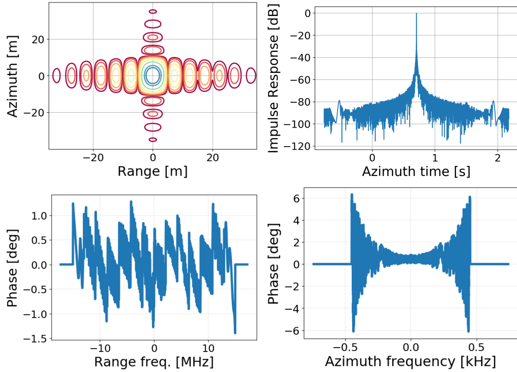
FIGURE 4.16: Polychromatic reconstruction approach using filter bank with sixteen band-pass filters.
