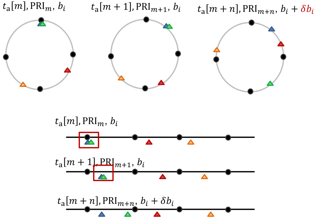
FIGURE 5.7: Coinciding sampling scheme with random PRI at three time instants showing the relocation of the samples in the sampling circle and azimuth time axis, and possible change in the relative distance between the samples due to drifts within the orbital tube. The colored triangles represent the input (received) data sampling positions and the black points represent the uniform output sampling grid.
