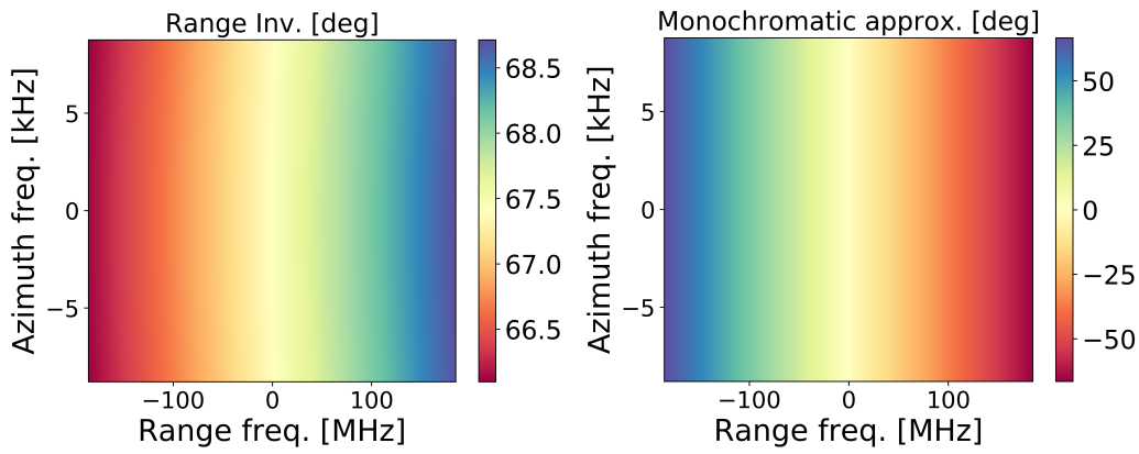
FIGURE 3.11: The left figure shows the difference in \Delta\Phi_i between two targets located at near and mid range ( T_1 and T_2 in Figure 3.9). The plot is computed as \Delta\Phi_i[f_r, f_a; r_0(T_1), b_i] - \Delta\Phi_i[f_r, f_a; r_0(T_2), b_i] and used to illustrate the contributions of the range variance in the modelling of the distributed sampling. The right figure shows the difference in \Delta\Phi_i due to the monochromatic approximation for the target located at the center of the swath (i.e., T_2 ) and is computed as \Delta\Phi_i[f_r, f_a; r_0(T_2), b_i] - \Delta\Phi_i[0, f_a; r_0(T_2), b_i] . The plots have been generated for a two-receiver X-band constellation with an along-track baseline of one kilometer and 15\lambda azimuth and range resolution.
