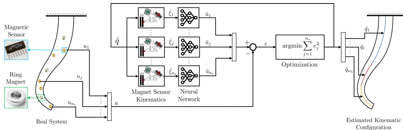
Fig. 1 Proprioception for continuum soft robots with magnetic sensors: an initial configuration estimate \hat{q} is employed to derive the kinematic relationship \xi between a sensor and each magnet. Subsequently, this kinematic description is used to predict the sensor measurements \hat{u} \in \mathbb{R}^{n_s} with a neural network trained in advance. A mean squared error (MSE) metric evaluates the accuracy of the predictions \hat{u} compared to the actual measurements u . Finally, we optimize the configuration estimate \hat{q} to achieve proprioception by minimizing the sensor measurement prediction loss.
