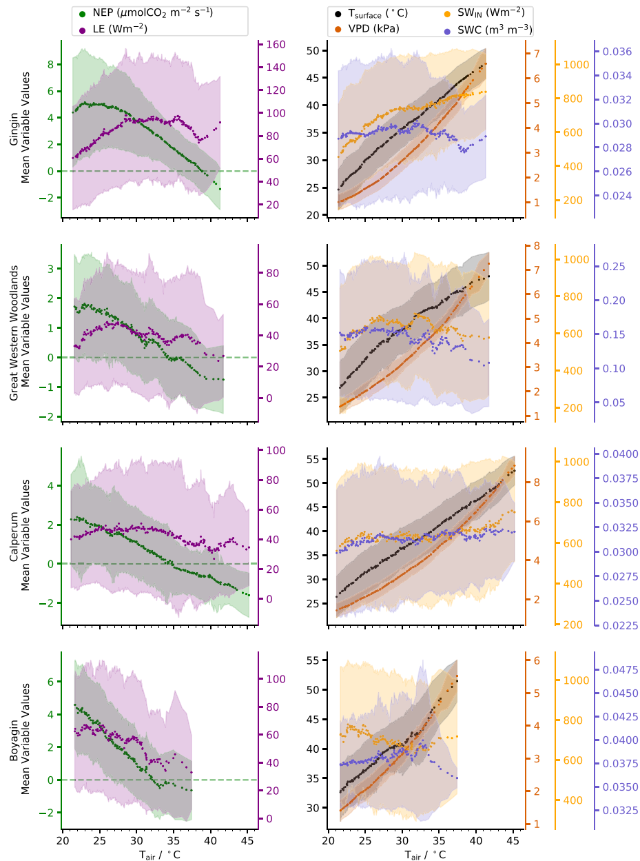
Figure 5. Mean and standard deviation of variables within each air temperature bin ( T_{\text{air}} ) of the four Australian woody ecosystems that show evidence of a decoupling. NEP: net ecosystem production, LE: latent heat, T_{\text{surface}} : estimated surface temperatures, VPD: vapour pressure deficit, SW_{\text{IN}} : shortwave incoming radiation, SWC: soil water content (0–15 cm).
