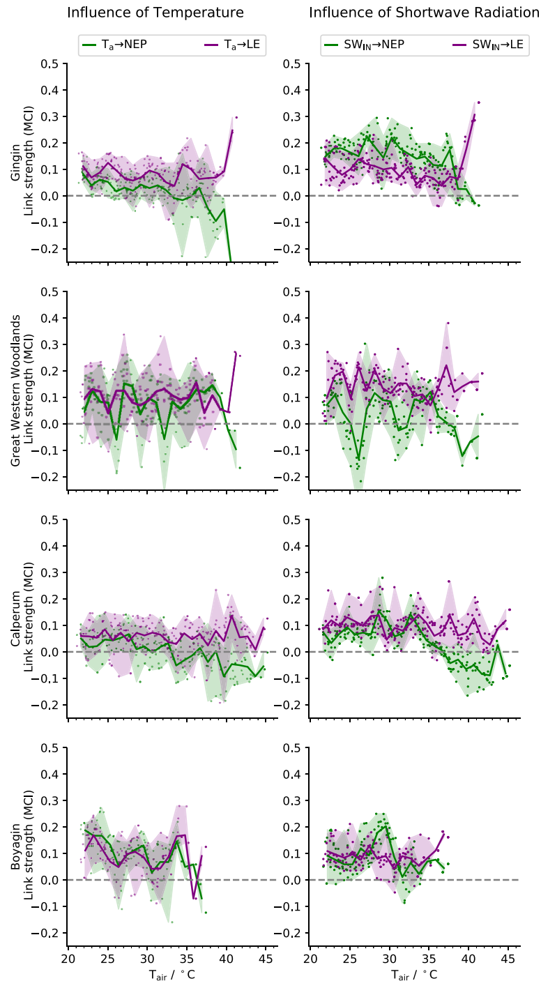
Figure 4. To further investigate the signs of decoupling that have emerged in the four ecosystems in figure 3, we plot the temperature behaviour. Shown are the link strength of incoming shortwave radiation ( SW_{IN} ) and air temperature ( T_{air} ) to net ecosystem production (NEP) and latent heat flux (LE) against mean T_{air} bin values. At a certain T_{air} (above 35 °C), the link strengths incorporating NEP and LE diverge.
