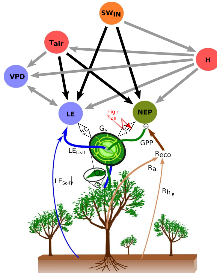
Figure 2. Investigated network structure between shortwave incoming radiation ( SW_{IN} ), air temperature ( T_{air} ), vapour pressure deficit (VPD), sensible heat flux (H), net ecosystem production (NEP) and latent heat (LE) (black and grey solid arrows). NEP is the sum of the two fluxes ecosystem respiration ( R_{eco} ) and gross primary productivity (GPP). R_{eco} itself contains autotrophic ( R_a ) and heterotrophic ( R_h ) respiration. LE is composed of evaporation from leaves ( LE_{Leaf} ) and surfaces ( LE_{Soil} ). As we mask precipitation events and subsequent measurements (according to the CSWI value, section 2.3), the top soil shall be rather dry which reduces contributions of LE_{Leaf} and R_h . LE and NEP are typically coupled via stomatal conductance ( G_s ) (dotted arrows). We hypothesise that the coupling between G_s and NEP breaks during high T_{air} as the leaf's temperature may reach critical levels if no precautionary measure is undertaken. This process will manifest in different responses of LE and NEP to SW_{IN} and T_{air} (black solid arrows). The dependence SW_{IN} \rightarrow NEP actually is indirect via GPP SW_{IN} \rightarrow GPP \rightarrow NEP . Thus we expect to circumvent influences of R_{eco} on NEP through the coupling SW_{IN} \rightarrow NEP and detect photosynthesis if it is active. Including VPD and H in the network structure allows to remove any detected influence on LE and NEP.
