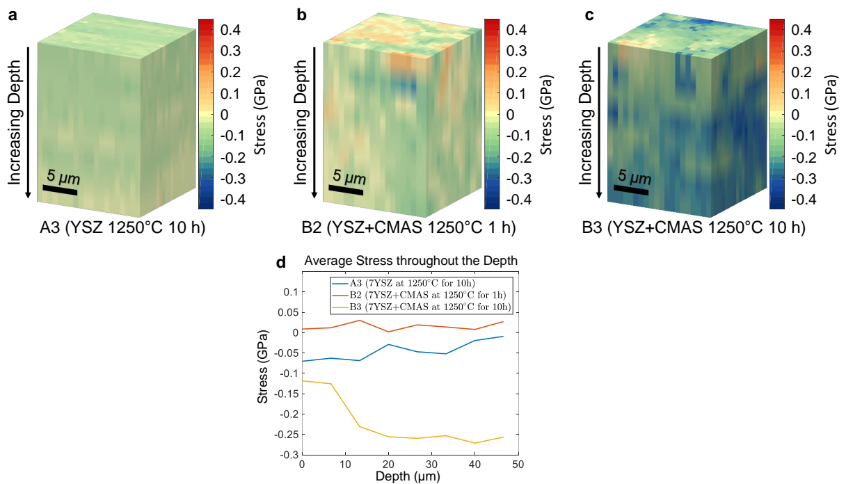
Figure 4: 3D reconstruction of the stress for the 643.78\text{ cm}^{-1} peak for (a) a non-infiltrated 7YSZ sample annealed at 1250°C for 10 h (A3), (b) a CMAS infiltrated 7YSZ sample annealed at 1250°C for 1 h (B2), and (c) a CMAS infiltrated 7YSZ sample annealed at 1250°C for 10 h. (d) Average stress as a function of depth for A3, B2 and B3.
