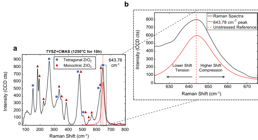
Figure 2: (a) Raman spectrum of CMAS infiltrated 7YSZ coating after an annealing time of 10 h at an annealing temperature of 1250°C. The associated Raman peaks for the tetragonal and monoclinic ZrO 2 phases are labelled with squares and triangles, respectively. (b) Expanded view of the tetragonal 643.78 cm -1 peak used within this study. Induced stresses are evaluated by the shifts with respect to this 643.78 cm -1 peak corresponding to the unstressed material. The coating at the probed point experiences a red shift and is in tension if the peak is shifted to a lower relative wavenumber with respect to the unstressed reference location. Similarly, the coating experiences a blue shift and is in compression if the peak is shifted to a higher wavenumber relative to the unstressed reference position.
