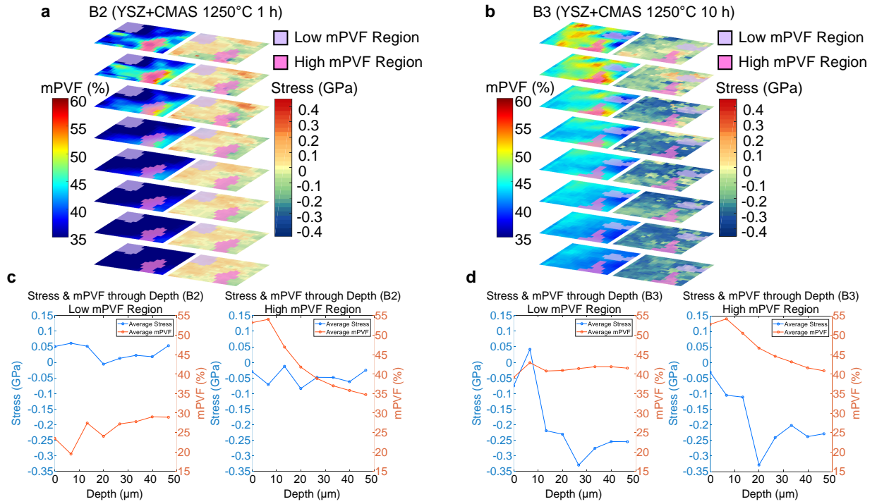
Figure 8: A comparison of the localized monoclinic phase concentrations, measured through the phase volume fraction (mPVF) [39], and the localized stress state of the probed areas throughout the probed depth of the coating are shown for samples infiltrated by CMAS annealed at 1250°C for (a) 1 h and (b) 10 h. For both samples, relatively low and high mPVF regions were selected and mPVF and stress were tracked within these regions throughout the depth of the coating for the (c) 1 h and (d) 10 h samples.
