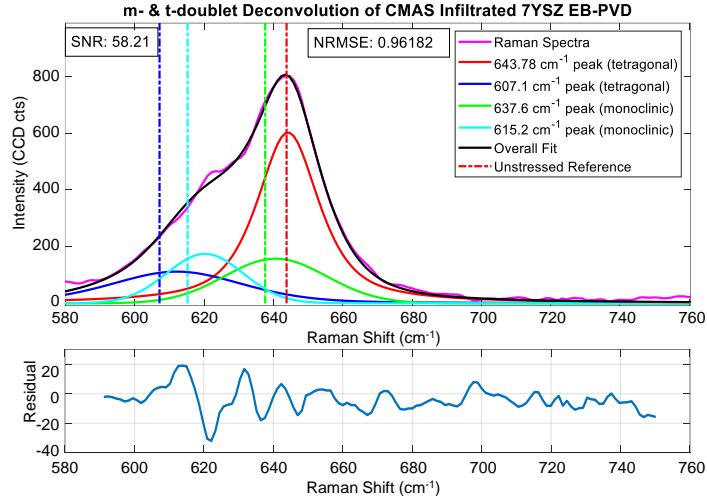
Figure 3: The deconvolution of the monoclinic (m) and tetragonal (t) doublets around the 643.78 \text{ cm}^{-1} peak. The measured Raman spectrum is shown in pink while the summation of the pseudo-Voigt function fitted peaks is in black. The unstressed reference peak positions of 607.1 , 615.2 , 637.6 , and 643.78 \text{ cm}^{-1} are marked in dashed lines corresponding to their respective fitted peak's colors of blue, cyan, green, and red, respectively. The unstressed reference peak positions are based on the findings in [42, 43]. The 607.1 and 643.78 \text{ cm}^{-1} peaks correspond to the tetragonal phase doublet while the remaining 615.2 and 637.6 \text{ cm}^{-1} peaks correspond to the monoclinic phase doublet. Additional measurement and goodness of fit parameters are also shown through the signal-to-noise ratio and the normalized root mean square equation goodness of fit, shown as SNR and NRMSE, respectively, in the figure. For the goodness of fit, 1.0 is an ideally perfect fit. The residual differences between the fitted and measured peaks are plotted in the lower graph.
