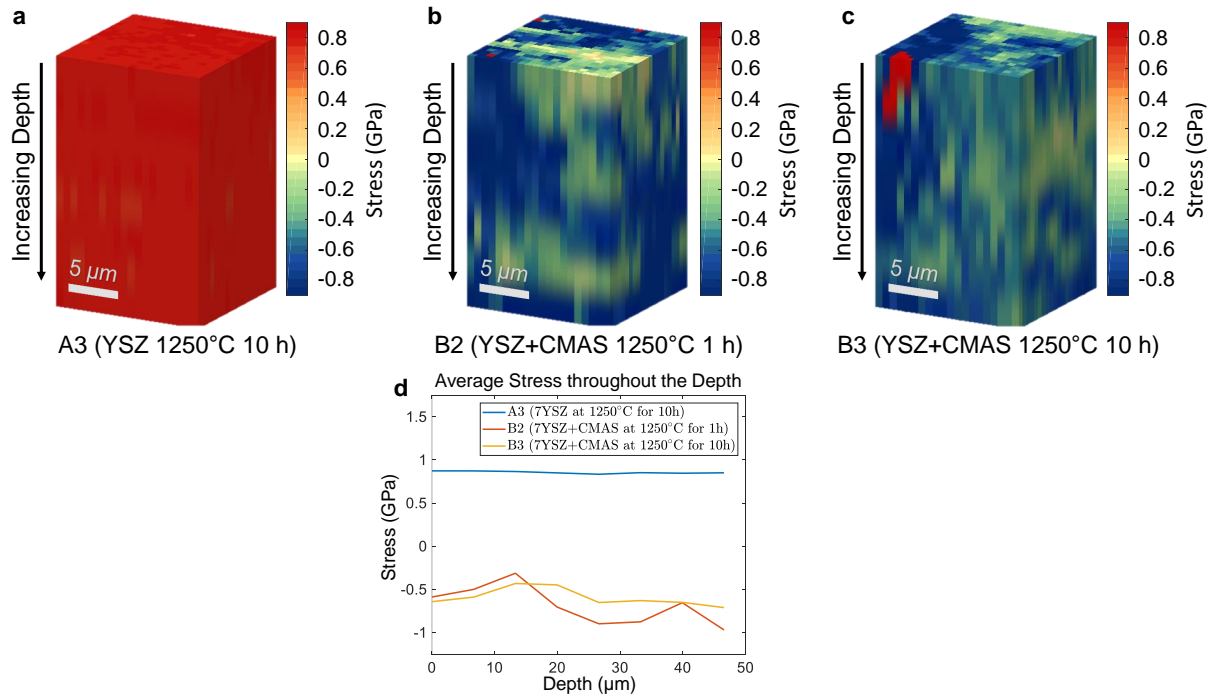
Figure 6: 3D reconstruction of the stress for the 463.7 \text{ cm}^{-1} peak for (a) a non-infiltrated 7YSZ sample annealed at 1250^\circ\text{C} for 10 h (A3), (b) a CMAS infiltrated 7YSZ sample annealed at 1250^\circ\text{C} for 1 h (B2), and (c) a CMAS infiltrated 7YSZ sample annealed at 1250^\circ\text{C} for 10 h (B3) as well as (d) the average stress as a function of depth for all three samples.
