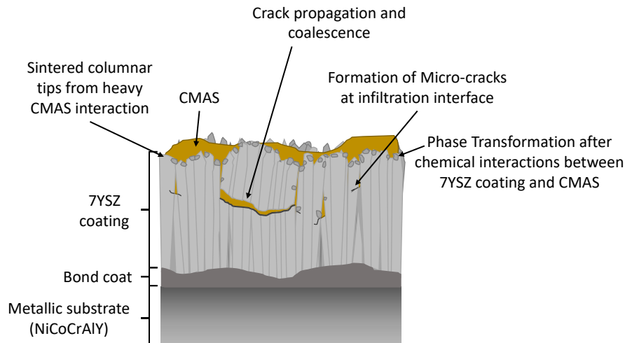
Figure 1: Schematic of a standard TBC composition, comprising of a metallic substrate, bond coat, and 7YSZ top coat, infiltrated by CMAS and some effects from this infiltration. These effects include the sintering of columnar tips and of the feather arms, micro-crack formation, propagation, and coalescence until causing localized coating delamination, and the localized formation of freely transformable ZrO_2 from the 7YSZ top coat.
