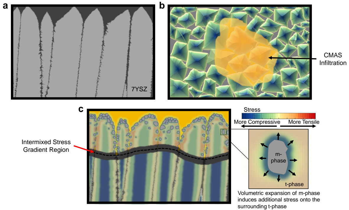
Figure 7: Schematics of (a) a pristine 7YSZ EB-PVD coating cross-section prior to any CMAS exposure or infiltration. (b) Top down view of the 7YSZ EB-PVD coating, showing cut aways of the columns as well as a region for CMAS infiltration. The typical stresses experienced by the coating is highlighted where compressive stresses are blue and slowly shift towards green until reaching a relatively unstressed state indicated in yellow. Stresses are scaled with high tensile stresses in red and are shifted to orange as the stresses approach a relatively unstressed state indicated in yellow. The stresses then slowly shift to green and finally blue as the stresses become more compressive. (c) is the cross-section of the 7YSZ EB-PVD coating after some time that CMAS as infiltrated and interacted with the coating, allowing for substantial monoclinic formation to occur. Two distinct regions form: the CMAS infiltrated and the non-infiltrated regions. An intermixed stress region forms at the interface between these two regions. The overall stress gradient within this intermixed region is dependent on several factors including, but not limited to, CMAS infiltration depth, coating age and the TGO growth development. The localized stress gradient induced by the formation of the monoclinic phase (m-phase) is highlighted to the right of (c) where compressive forces, relative to the surrounding tetragonal phase of the coating, are present around the globular monoclinic phase.
