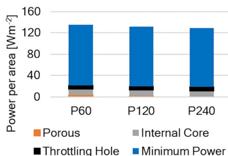
Fig. 21 Comparison of suction power for different porous sheets
