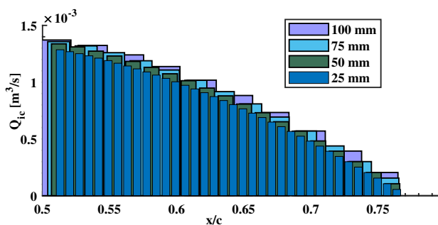
Fig. 22 Variation of volume flow rate inside internal core for different cell width
