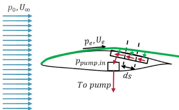
(a) Airflow path in xHLFC suction system
