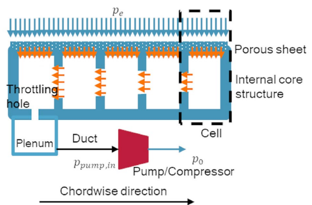
(b) Flow in the internal structure of xHLFC suction system
