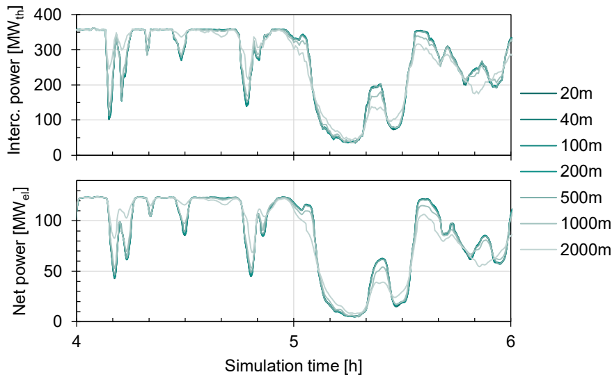
Figure 2. Excerpt of simulated intercept (top) and net (bottom) power based different Cartesian cluster/pixel sizes.
