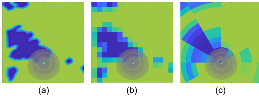
Figure 1. Visualization of (clustered) DNI maps and heliostat field layout (a: original pixels 20 m by 20 m; b: Cartesian clustering 500 m by 500 m; c: polar clustering 30 ° by 500 m).
