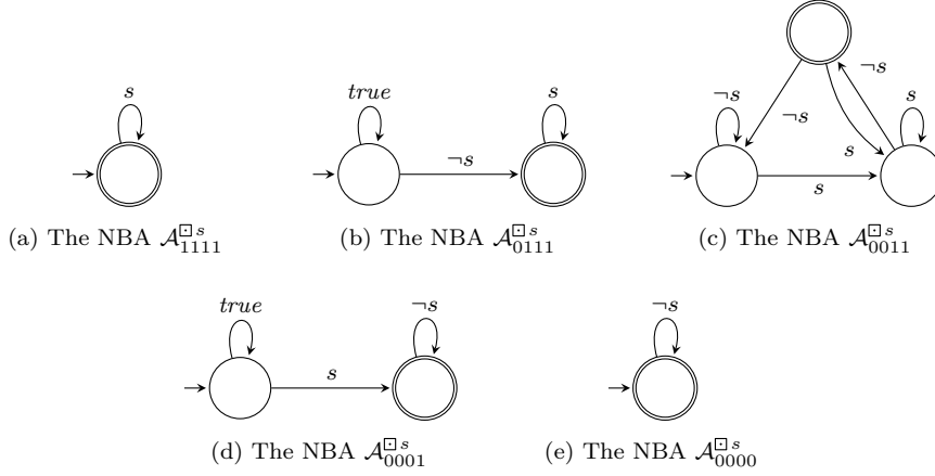
Fig. 1: The Büchi automata \mathcal{A}_\beta^{\square s} constructed in Step 1 of our monitor construction
