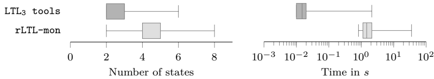
(b) Analysis of the monitor construction for the 54 formulas that are both LTL-monitorable and rLTL-monitorable
