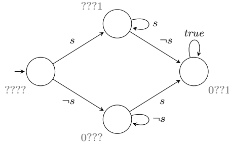
Fig. 4: The final monitor \mathcal{M}_{\square s}
