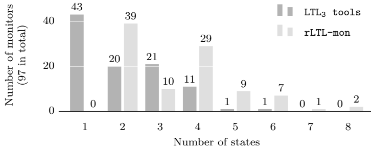
(a) Histogram of the number of monitors with respect to their size
