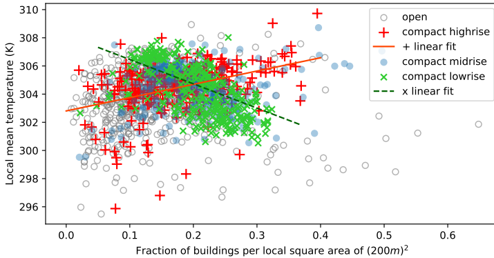
Fig. 5. Local temperature dependency on building density in New York City for selected local climate zones.
