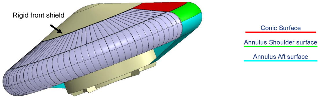
Figure 11: EFESTO IAD architecture for Mars application.
