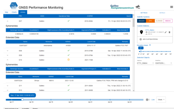
Fig. 5. The satellite library with details displayed for E07 and E10. Note how the status of newly launched GSA0224 is still set to testing while other Galileo satellite are healthy and operational.
