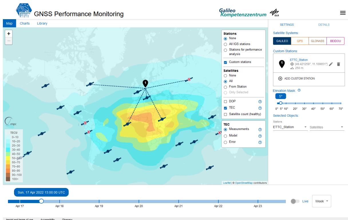
Fig. 6. Ionospheric conditions around lunch time on 2022-04-17.
