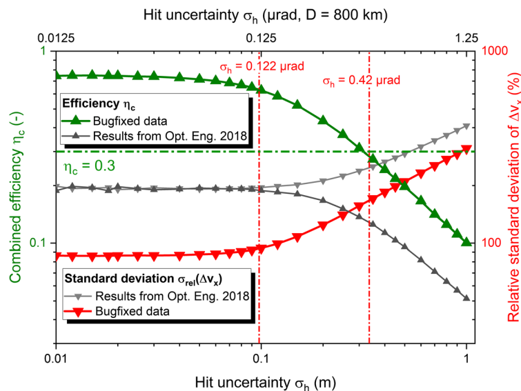
Fig. 1 Combined efficiency \eta_c and relative standard deviation \sigma_{\Delta v_{ax}}/\langle\Delta v_{ax}\rangle of the axial velocity increment: dependency on hit uncertainty. Comparison of simulation results shown in Fig. 8 of Opt. Eng. 58(1), 011004 (2018) with revised data after numerical bugfixing.
