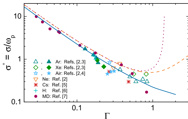
Fig. 1. Reduced conductivity of a moderately non-ideal ( \Gamma \sim 0.02 - 2 ) fully ionized plasma as a function of the coupling parameter \Gamma . Symbols correspond to experimental results and MD simulations (see the legend). Dotted line corresponds to the weakly coupled limit of the conventional Coulomb logarithm, dashed line to the unsimplified conventional Coulomb logarithm, and the blue solid line to the modified Coulomb logarithm. For details see Ref. [1].
