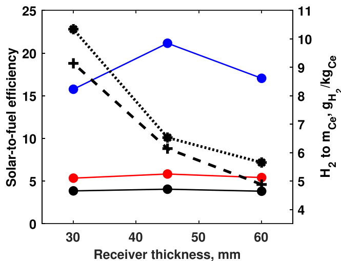
Fig. 19. Solar to fuel efficiency (black - normal \eta_{sf} , red - with heat recovery \eta_{sf, HR} , blue - ideal \eta_{sf, ideal} ) and H_2 produced per ceria mass loading (dashed - actual, dotted - maximum) versus the absorber thickness.
