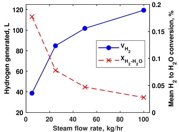
Fig. 9. Amount of hydrogen produced and mean H_2 to H_2O conversion extent as a function of the steam flow rate for the first cycle. T_{red, end} = 1100 \text{ °C} , f_{CeO_2} = 25\% , V_{H_2, ideal} = 131.876 \text{ L} .
