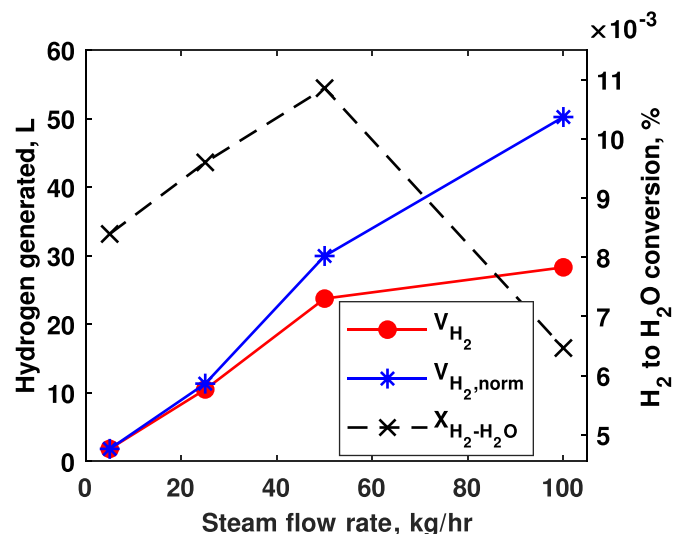
Fig. 10. Amount of hydrogen produced and mean H_2 to H_2O conversion extent as a function of the steam flow rate for the second cycle. T_{red, end} = 1100 \text{ °C} , \phi_{CeO_2} = 25\% . V_{H_2, norm} is the amount of hydrogen normalized by the ratio of the ideal H_2 production for each case to the 5 \text{ kg h}^{-1} case.
