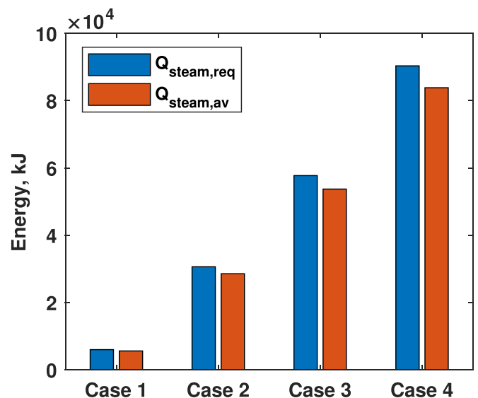
Fig. 13. Energy required for steam generation compared to energy available in the H_2/H_2O mixture at outlet, for case 1–4.
