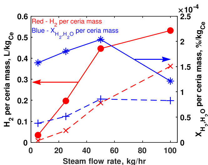
Fig. 12. Generated hydrogen and mean H_2 to H_2O conversion extent normalized per ceria mass as a function of the steam flow rate for the second cycle in Case 1 to Case 4 (solid line: \phi_{ce} = 25\% , dashed line: \phi_{ce} = 100\% ).
