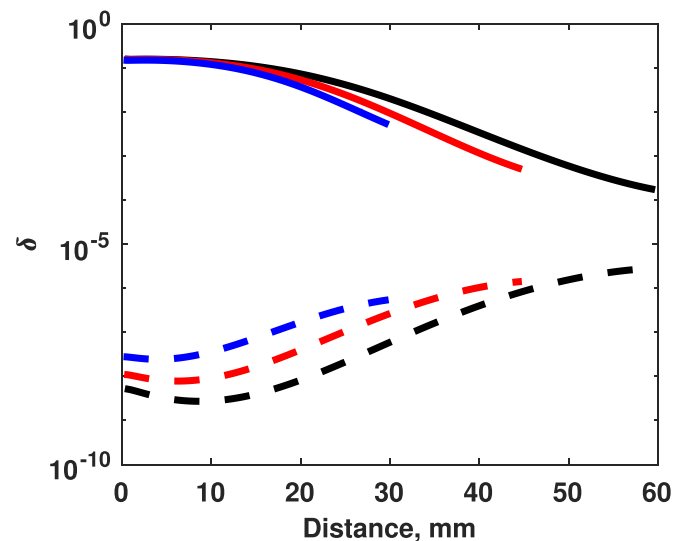
Fig. 20. Nonstoichiometry extent profiles across the receiver for various absorber thickness at the start and end of the reduction step (solid lines - reduction end, dashed lines - reduction start). Black - absorber thickness 60 mm, red - absorber thickness 45 mm, blue - absorber thickness 30 mm.
