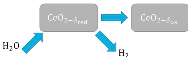
Fig. 1. Solar-driven 2-step reduction–oxidation cycle for water splitting.
