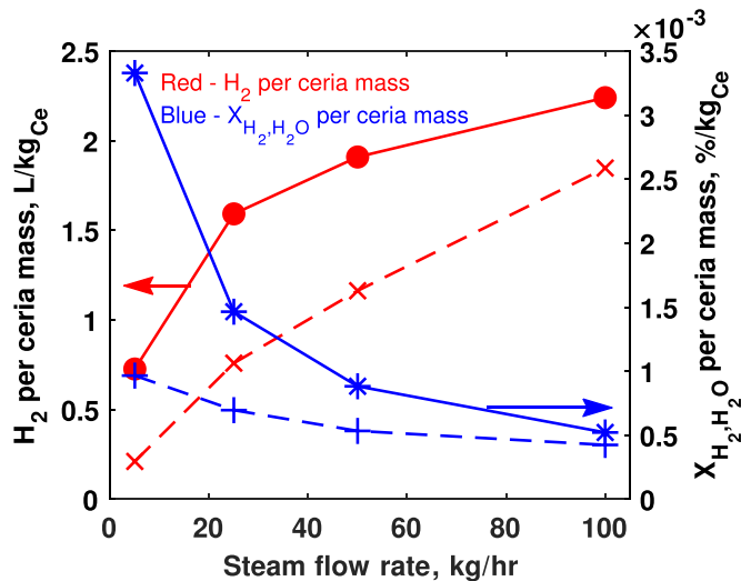
Fig. 11. Generated hydrogen and mean H_2 to H_2O conversion extent normalized per ceria mass as a function of the steam flow rate for the first cycle in Case 1 to Case 4 (solid line: \phi_{ce} = 25\% , dashed line: \phi_{ce} = 100\% ).
