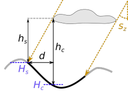
Figure 17. Principle of the measurement of cloud- and shadow-borders
