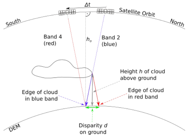
Figure 2. Principle of acquisition geometry of image bands separated in a FPA; h_o : height of the orbit, \Delta t : time lag as listed in table 1.
