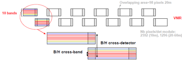
Figure 3. Focal plane assembly of Sentinel-2
