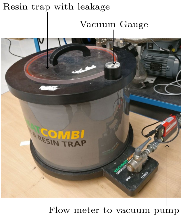
Fig. 8 Resin trap: experimental setup
