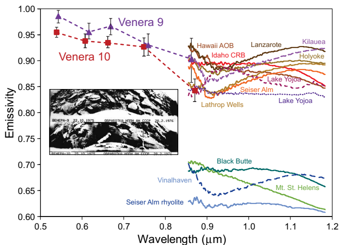
Fig. 1. Laboratory emissivity data obtained at 440^{\circ}\text{C} sample temperature (solid lines) compared to multispectral data from the Venera 9 and 10 landers [reflectance converted to emissivity with associated error bars digitized from figure 8 of Ekonomov et al. (18)]. Dashed lines indicate particles with ranges of grain sizes: 700 to 1000 \mu\text{m} (long dashes), >500 \mu\text{m} (medium dash), and 250 to 500 \mu\text{m} (dots). This is the first direct spectral confirmation that Venera 9 and 10 landed on basaltic material. The inset shows images of the landing site obtained by the Panoramic Telephotometer [Venera 9–NASA Space Science Data Coordinated Archive (NSSDC) dataset ID (photo): 75-050D-01A; Venera 10–NSSDC dataset ID (photo): 75-054D-01A]. The spectra were obtained in both cases on the opposite side of the lander.
