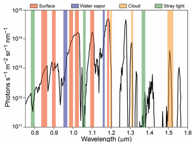
Fig. 4. Wavelengths of bands used opportunistically around gaps in the \text{CO}_2 atmosphere of Venus (54). Collectively, these offer a comprehensive sampling of surface, water vapor cloud opacity, and stray light, as needed to estimate errors on surface bands. The black line is an observed nightside emission spectrum of Venus.
