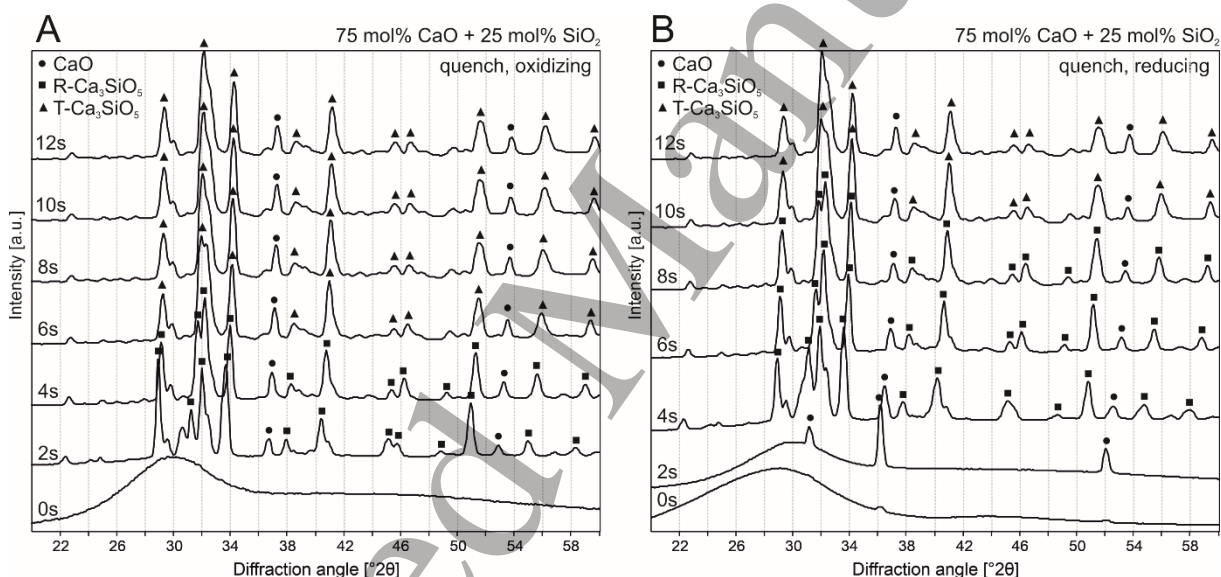
Figure 5: Detail of X-ray diffractograms (20-60 °2θ) of quenched samples from mixture II under A) oxidizing conditions and B) reducing conditions. The time point 0 was set to the last diffraction pattern before crystallization.
