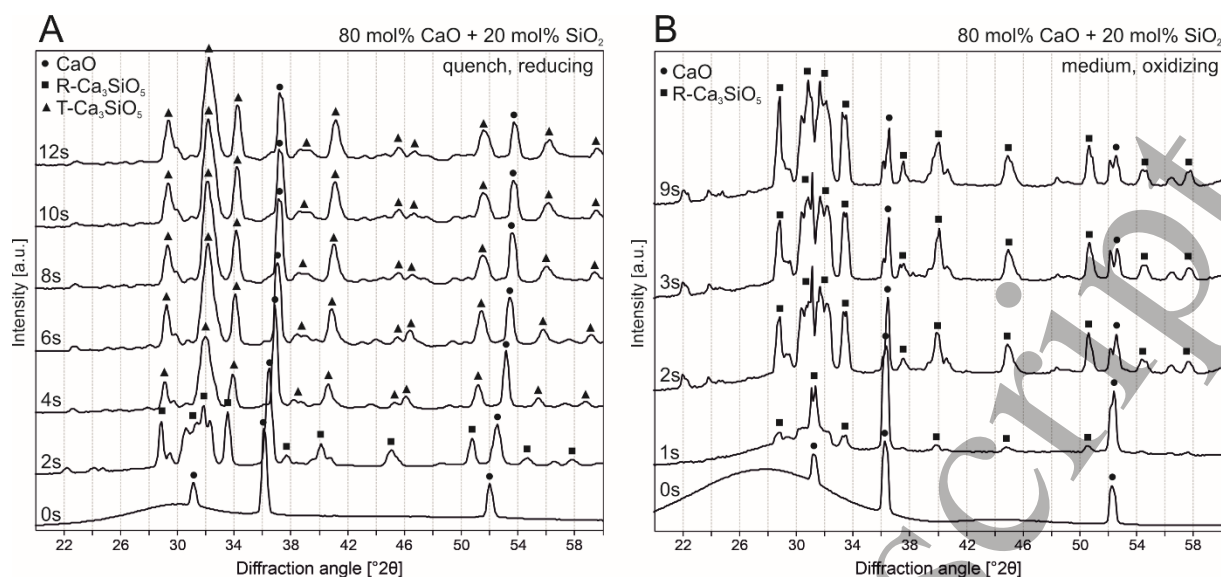
Figure 3: Detail of X-ray diffractograms (20–60 °2θ) of samples from mixture I. A) Diffractograms from the first 12 s after quenching under reducing conditions. B) Diffractograms from the first 9 s medium cooling under oxidizing conditions. The time point 0 was set to the last diffraction pattern before \text{Ca}_3\text{SiO}_5 crystallization.
