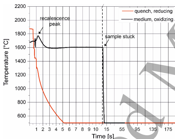
Figure 4: Temperature curves of samples from mixture I during cooling, measured with a pyrometer. The time point 0 was set to one second before crystallization of \text{Ca}_3\text{SiO}_5 .
