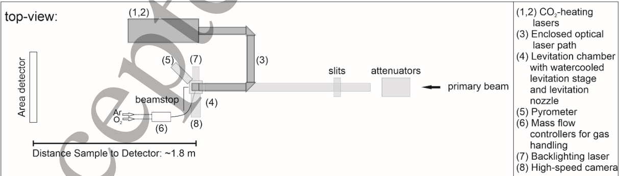
Figure 2: Sketch of the aerodynamic levitation setup at beamline P21.1 at DESY. The sketch shows a top view on to the x-y-z stage. Sample installation is carried out via the beam-exit window to the levitation chamber. To this end the beamstop is moved to its end-position to provide free-access to the levitation chamber and nozzle onto which the sample is mounted.
