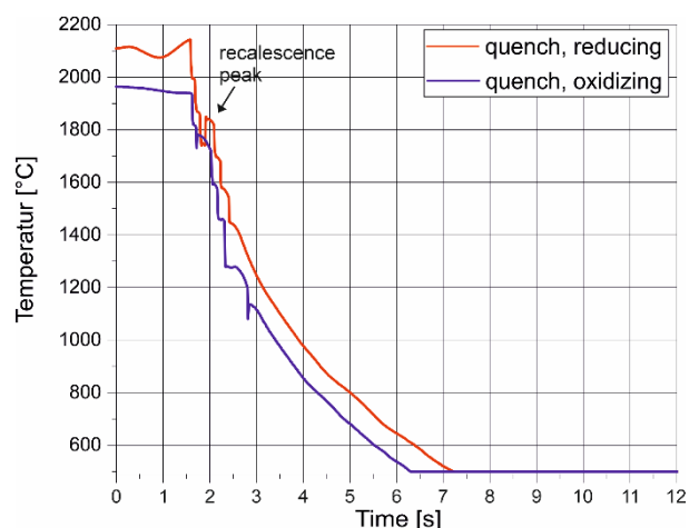
Figure 6: Temperature curves of quenched samples from mixture II, measured with a pyrometer. The time point 0 was set to one second before crystallization.
