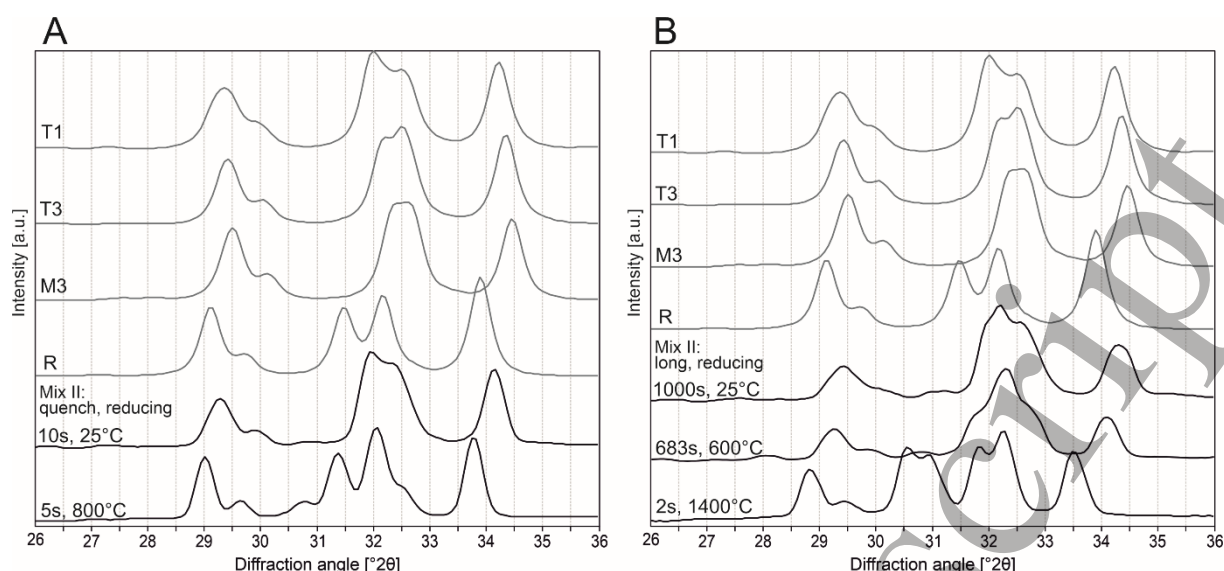
Figure 13: Comparison of the angular region 26-36 °2θ of the reference R (Nishi and Takéuchi 1984) (COD 8104367), M3 (Nishi et al. 1985) (COD 9008366), T3 (De La Torre et al. 2008) (COD 9016125) and T1 (Golovastikov et al. 1975) (COD 9014362) with A) a sample of mixture II quenched under reducing conditions and B) a sample of mixture II slowly cooled (1.6 °C/s) under reducing conditions at high temperatures and at room temperature. The specified times refer to the time elapsed after the last recorded diffractogram in the molten state.
