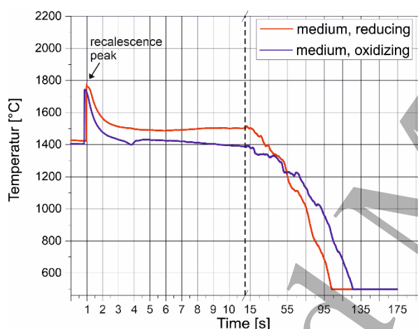
Figure 8: Temperature curves of medium cooled samples from mixture II, measured with a pyrometer. The time point 0 was set to one second before crystallization.
