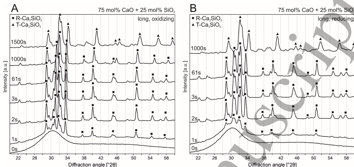
Figure 9: Detail of X-ray diffractograms (20-60 °2θ) of slowly cooled samples from mixture II under A) oxidizing conditions and B) reducing conditions. The time point 0 was set to the last diffraction pattern before crystallization.
