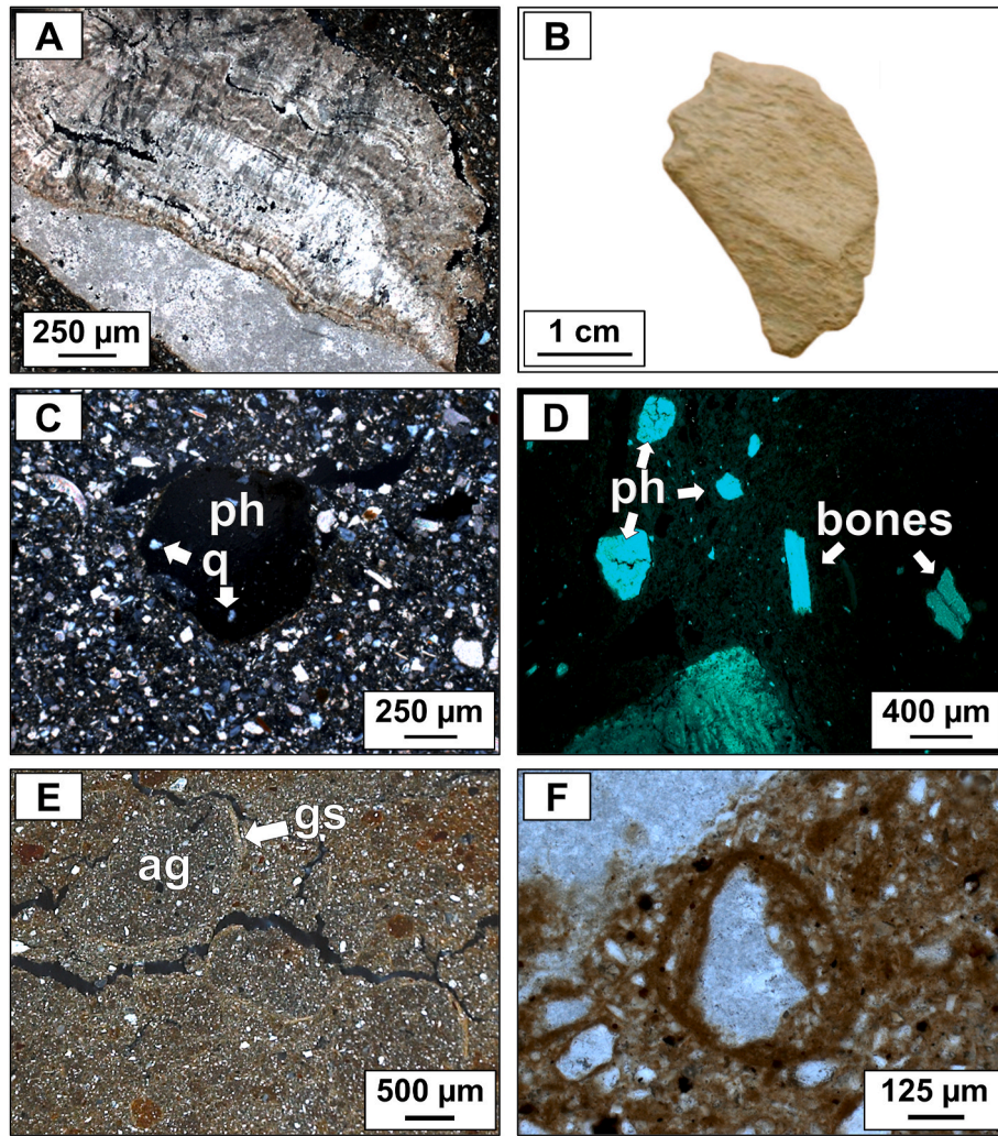
Fig. 4. Evidence of cave and landscape erosion from Ach and Lone Valley/Lone Valleys. Speleothem (A) and bone fragment (B) from Hohle Fels, grains of phosphatized loess (C) and bones (D) from Bockstein, cryogenic features (E and F) from the hillside opposite Hohlenstein-Stadel.
