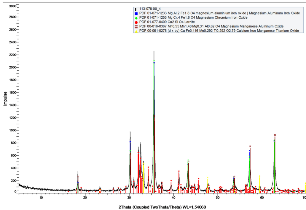
Figure S2. X-ray diffraction (XRD) pattern of the cycled powder made of sintered slag pebbles.
