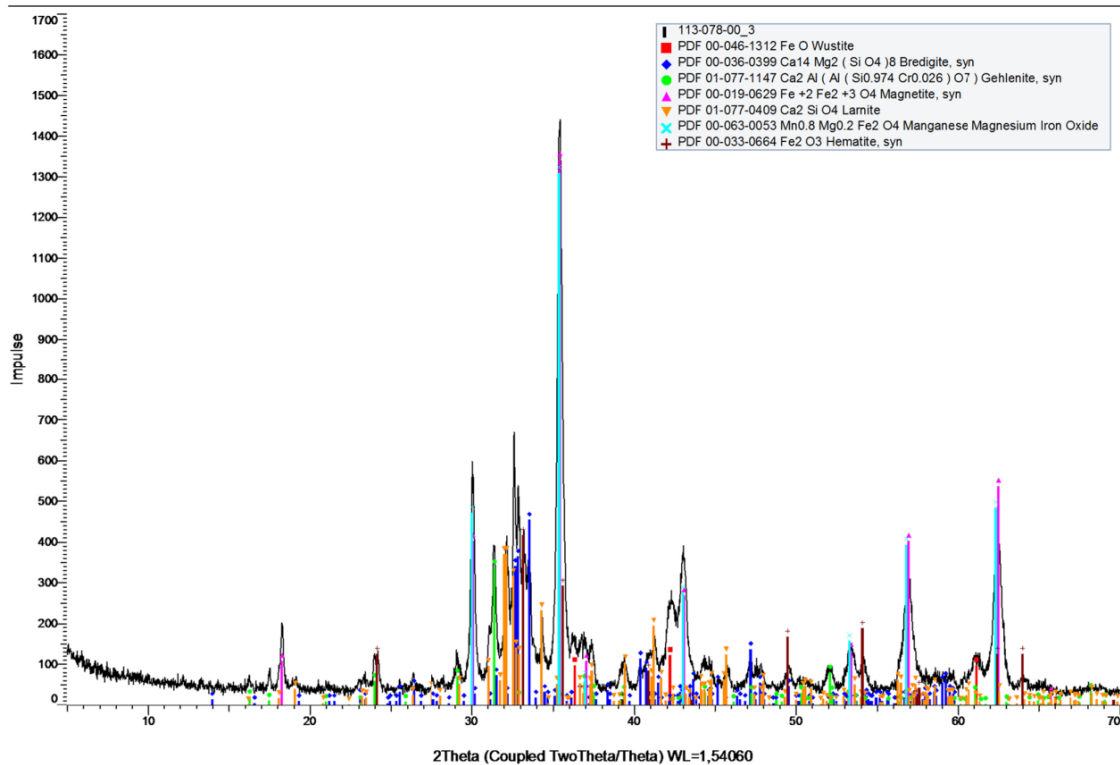
Figure S4. X-ray diffraction (XRD) pattern of the cycled powder made of raw slag.
