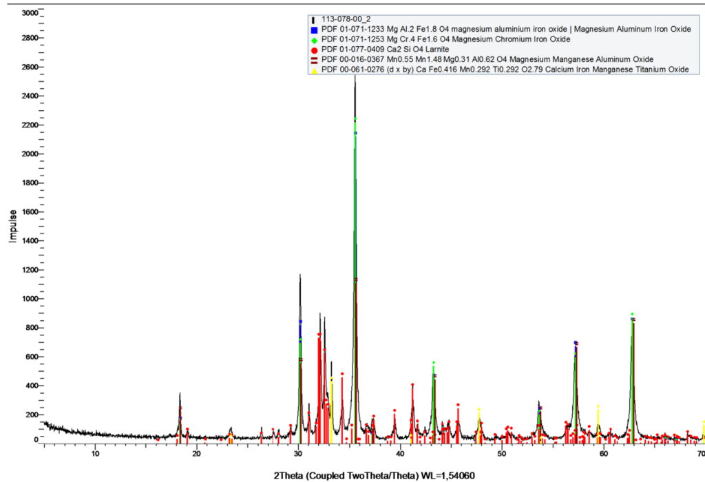
Figure S3. X-ray diffraction (XRD) pattern of the non-cycled powder made of sintered slag pebbles.
