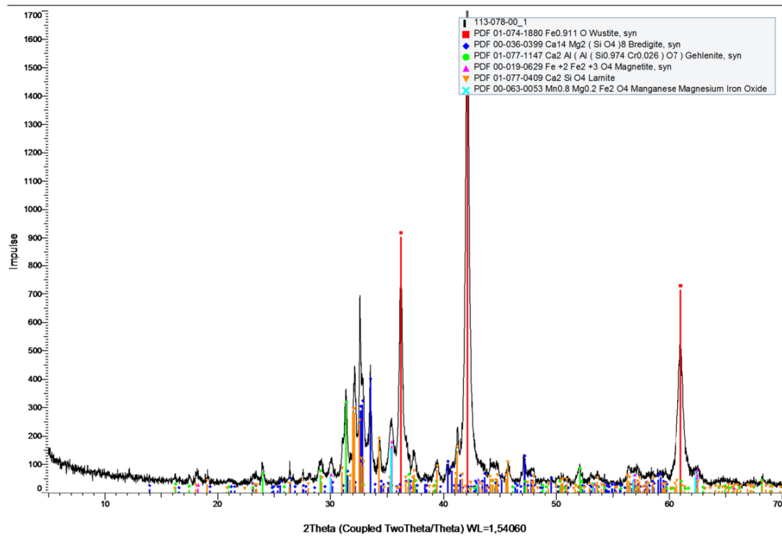
Figure S5. X-ray diffraction (XRD) pattern of the non-cycled powder made of raw slag.
