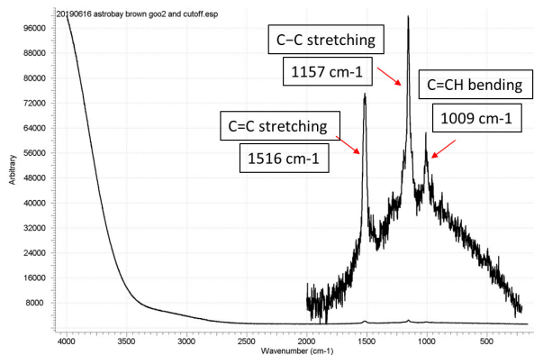
Fig. 3: Example Raman spectra showing high fluorescence after 3500\text{cm}^{-1} and a typical carotenoids' signature (zoomed in part shown above) with peaks at 1009 , 1157 and 1516\text{cm}^{-1} corresponding to C=CH bending, C=C stretching and C=C stretching modes, respectively.
