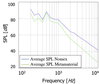
(b) Comparison of the average Sound Pressure Level (SPL) for all the head acoustic cavities of the fuselage for two different core materials.
