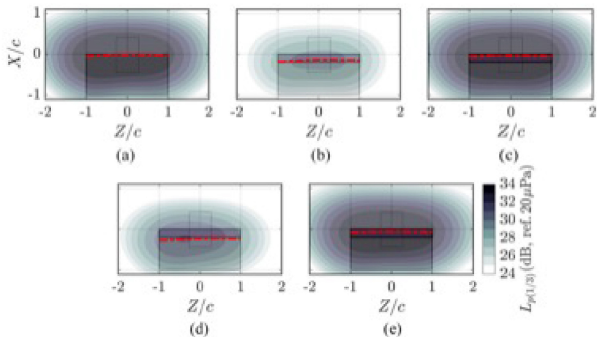
Fig. 1. Source maps for the one-third octave band with f_c = 1000 Hz for the measured test cases. (a) Solid. (b) Permeable with 450 \mu\text{m} foam cell diameter. (c) Nonpermeable Permeable with 450 \mu\text{m} foam cell diameter. (d) Permeable with 800 \mu\text{m} foam cell diameter. (e) Nonpermeable Permeable with 800 \mu\text{m} foam cell diameter.
