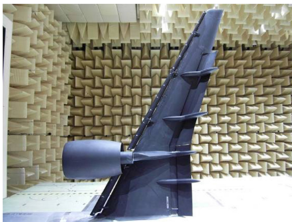
Fig. 6. Half-span wing model in anechoic test section of DNW-NWB wind tunnel.
