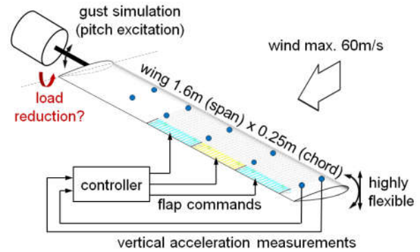
FIGURE 21 Set-up of the wind tunnel experiment
