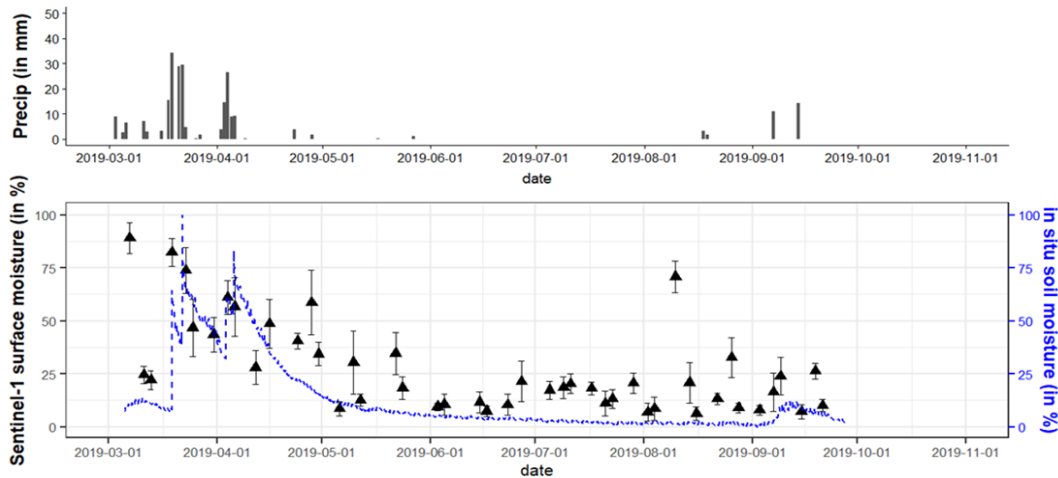
Fig. 5: Sentinel-1 SurfMI and in situ soil moisture and precipitation time series for the Kruger National Park (Precipitation Data provided by SANParks Data Repository).
