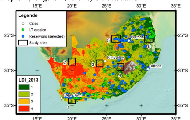
Fig. 1: SALDi study sites (black blocks). The map shows the study sites based on the Land Degradation Index map 2013 (LDI_2013, 1 = slight to 4 = severe, from: ARC 2017), the selected dams for an update of the reservoir siltation and sediment yield assessment of [9], as well as the currently available data on long-term erosion rates
