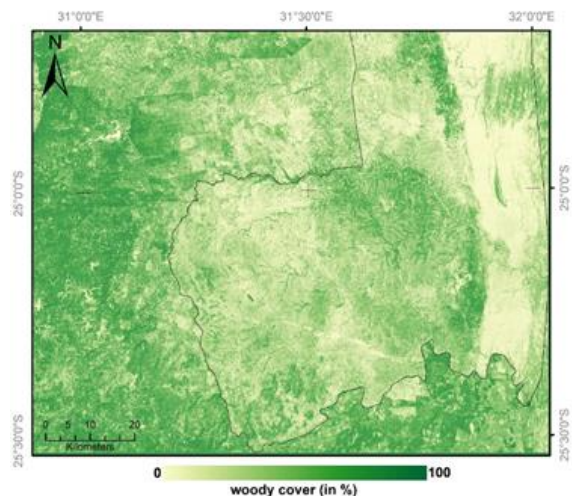
Fig. 2: Sentinel-1 derived woody cover map of the southern part of the KNP with a spatial resolution of 10m for the years 2016/17.
