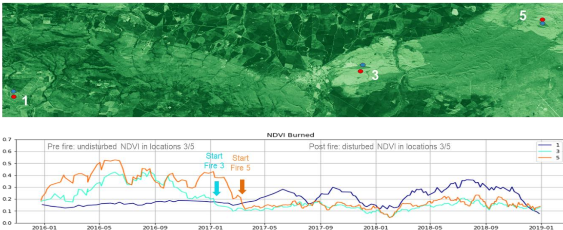
Fig. 3: NDVI time series based on Sentinel 2 data of fires in Cape Agulhas region: Fires 3 and 5 occurred in the beginning of 2017 and exhibit a slow recovery. Fire 1 started before 2016 and slowly recovered during 2017 and 2018 but does not reach NDVI values comparable to pre-fire levels at sites 3 and 5, probably indicating onset of land degradation.
