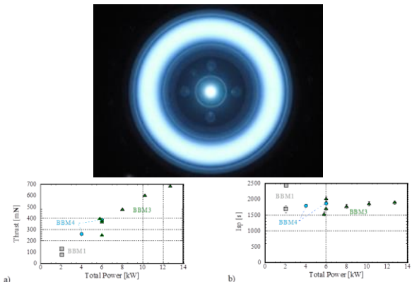
Fig. 11. Above: 6 kW Japanese Xenon HET (Breadboard model (BBM) testing at JAXA.). Below a) to b): thrust and Isp as a function of power for three BBM. BBM4 obtained 393 mN and 1,940s at the beginning of life test [22], and as a result of preliminary life test [22], it is found that Isp and thrust efficiency decreased from 1940 s and 62.9% to reach the constant values of about 1,900s and 60%, respectively. During accumulated operation from 1,012 to 4,048 hours, nearly constant performance continued [23].
