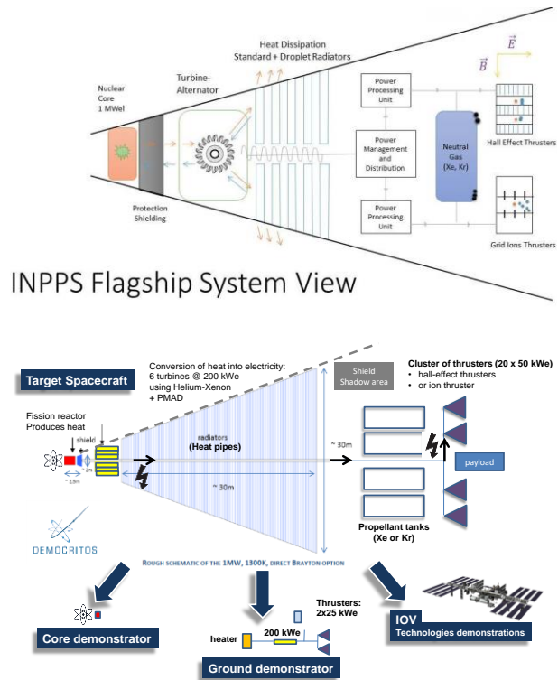
Fig. 1. Top: INPPS as a space system with its sub-systems. Bottom: INPPS flagship principle scheme, characteristics of sub-systems and DEMOCRITOS demonstrator characteristics. Courtesy of CNES / European-Russian DEMOCRITOS project [1] and [3].
