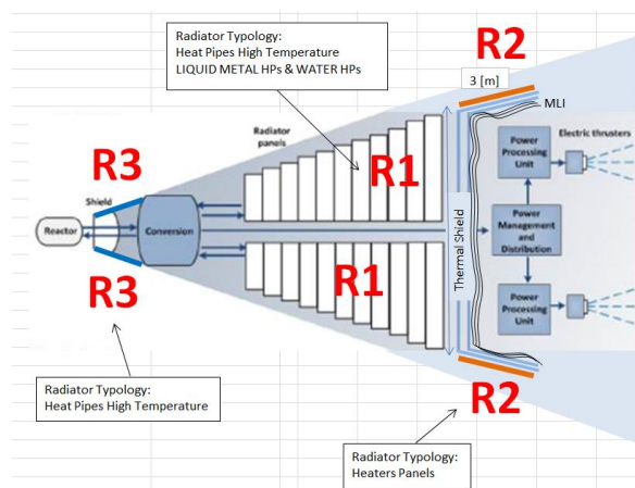
Fig. 4 DEMOCRITOS radiator demands. Due to successful MW reactor tests in Russia, R1 will consist of standard plus droplet radiators in a re-designed INPPS flagship (2020).
