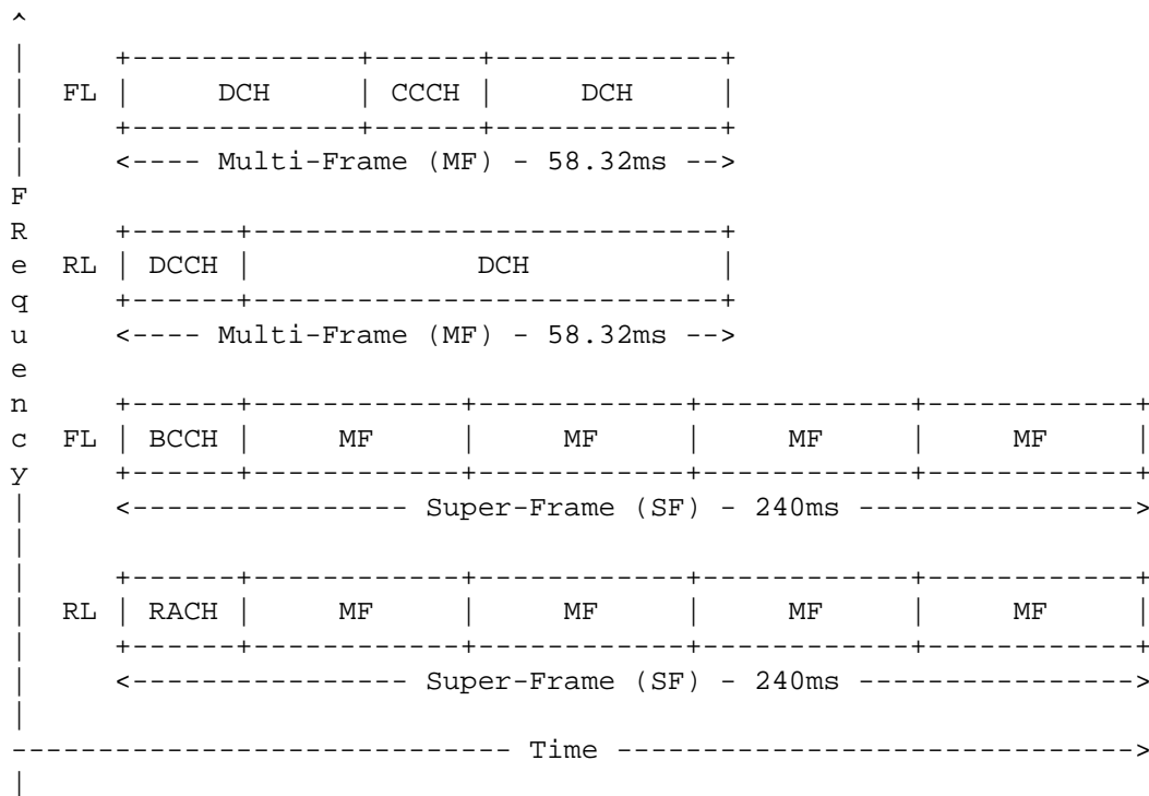
Figure 4: LDACS frame structure
