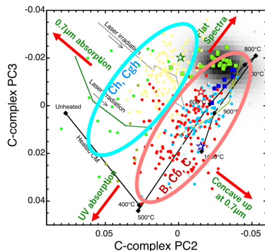
Fig. 5. Comparison in principal-component scores (PC2-PC3) between Ryugu regolith (black) and boulders (yellow) with main-belt C-complex asteroids [7], Murchison samples with heating (black line [8] and laser-irradiation (light green [9] and grey lines [8]) experiments are shown with Parent bodies, Polana (blue star), Eulalia (red star), and Erigone (green star).
