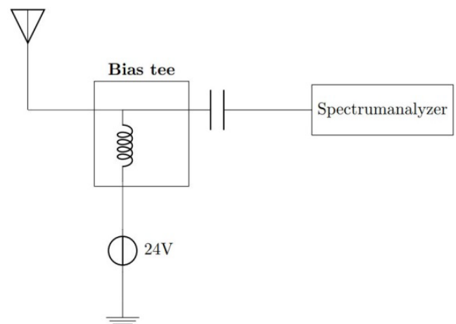
Figure 4. Used setup for field strength measurement.
