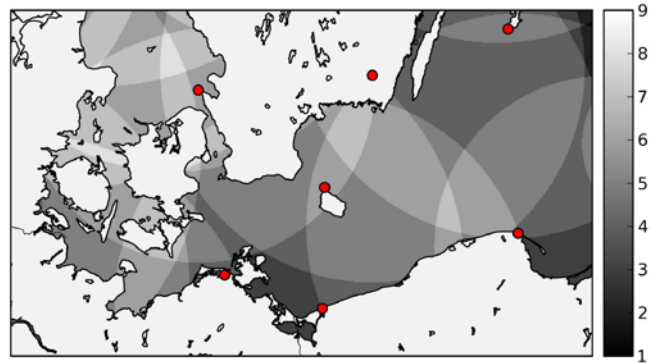
Figure 2. Number of available radio beacon signals calculated with nominal range of beacons.
