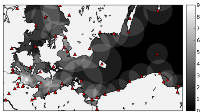
Figure 3. Number of available AIS base station signals calculated with base station antenna height.
