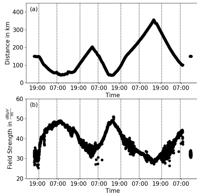
Figure 6. Distance over time (a) and field strength over time (b) for the German transmitter station Groß Mohrdorf. The dotted lines indicate times of sunrise or sunset.
