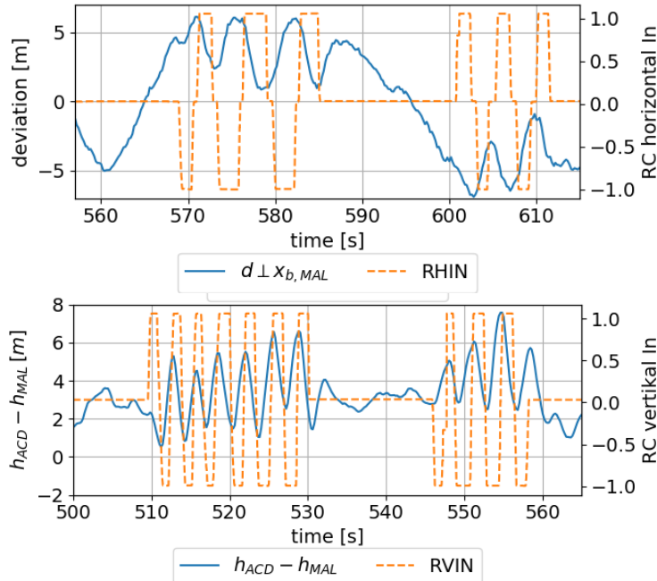
Figure 9: Horizontal (top) and vertical (bottom) displacement during control inputs [13]
