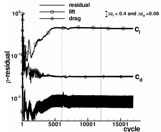
Fig. 4 Convergence history of the RANS computation, low Reynolds number landing case, dotted: transition prediction start, dashed: transition prediction end.
