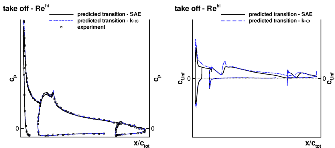
Fig. 18 c_p - and c_f -distributions, high Reynolds number take-off case, Wilcox k-\omega turbulence model.
