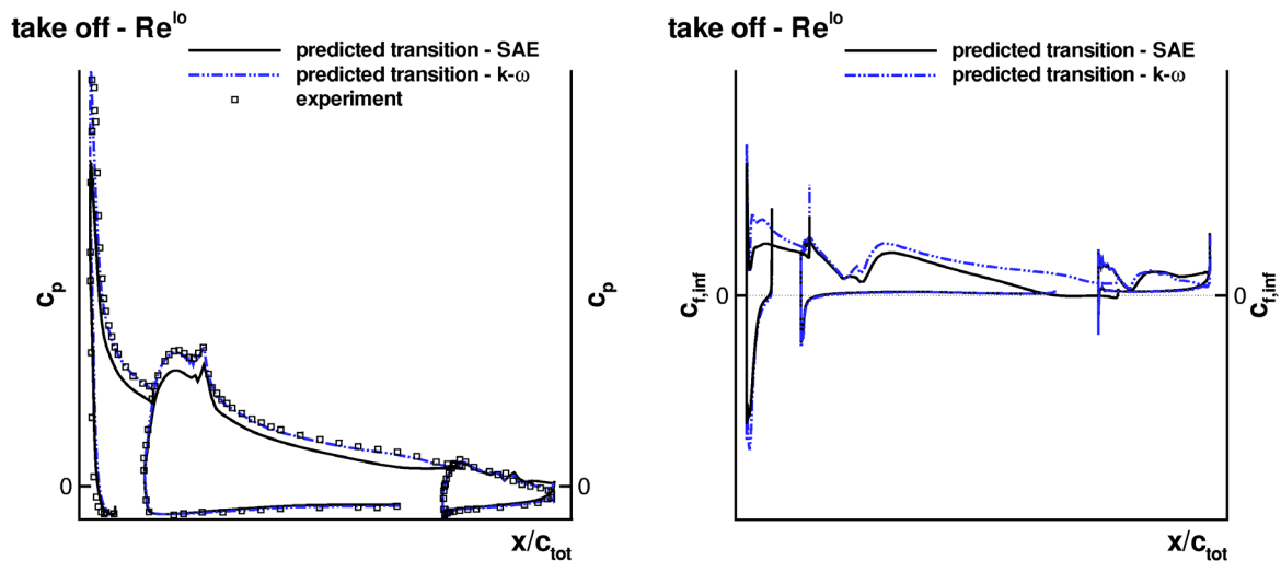
Fig. 17 c_p - and c_f -distributions, low Reynolds number take-off case, Wilcox k-\omega turbulence model.
