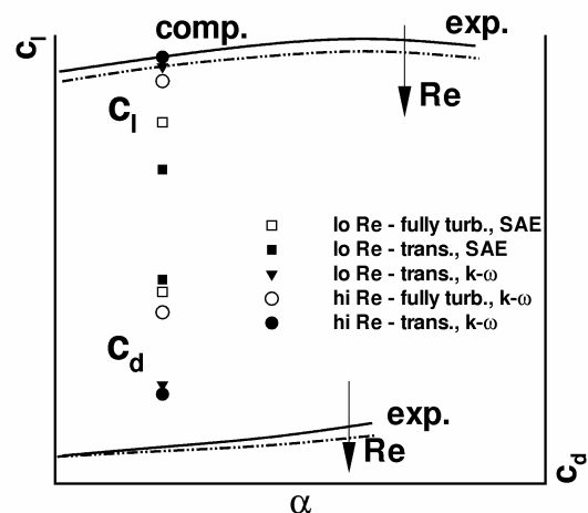
Fig. 19 Measured and computed lift coefficients, c_l , and drag coefficients, c_d , versus the angle of attack \alpha , take-off case.
