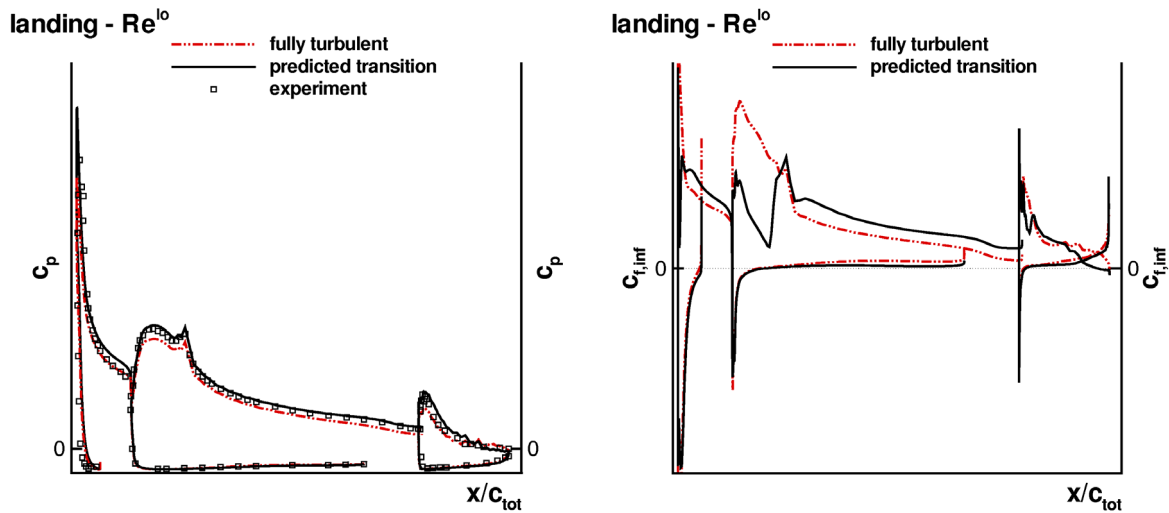
Fig. 15 c_p - and c_f -distributions, low Reynolds number landing case, Wilcox k-\omega turbulence model.
