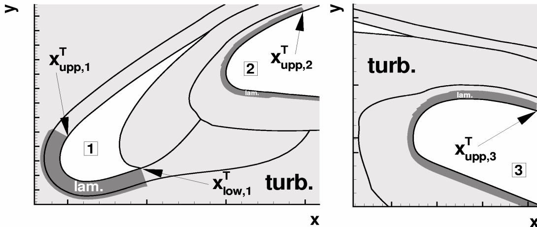
Fig. 3 Laminar zones of a two-dimensional three-element airfoil configuration in a turbulent remainder of the flow domain, point transition, slat and main airfoil (left), flap (right).
