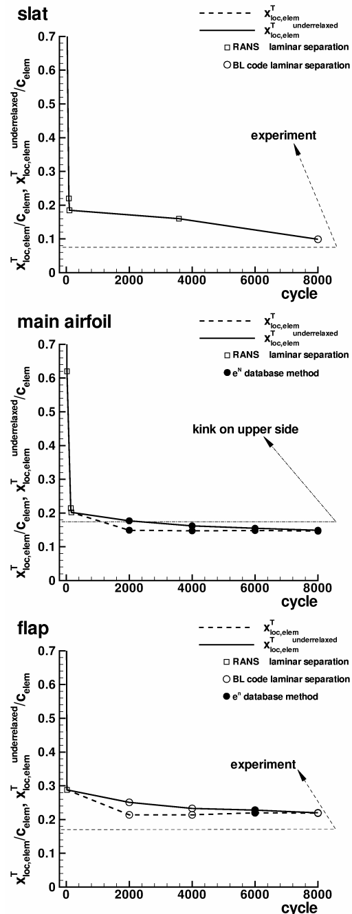
Fig. 10 Convergence histories of the transition location iteration at the slat, main airfoil and flap, high Reynolds number take-off case.
