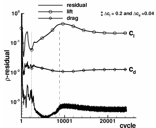
Fig. 6 Convergence history of the RANS computation, low Reynolds number take-off case, dotted: here the transition prediction process had started, long dashed: here the restart run started using fixed predicted transition locations.
