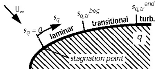
Fig. 2 Stylised depiction of laminar, transitional and turbulent flow regions at surface side q .
