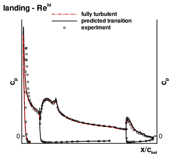
Fig. 21 c_p -distributions, high Reynolds number landing case, Wilcox k-\omega turbulence model, experimental distribution taken at the cleaned wind tunnel model with attached flow over the flap.
