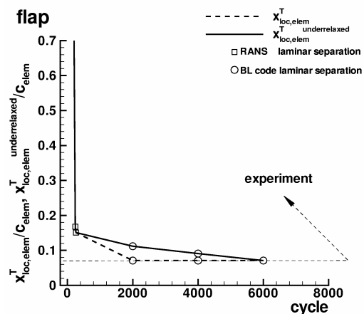
Fig. 12 Convergence histories of the transition location iteration at the slat, main airfoil and flap, high Reynolds number landing case.
