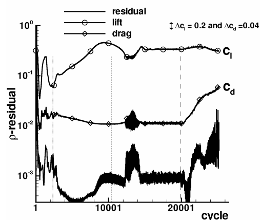
Fig. 5 Convergence history of the RANS computation, low Reynolds number take-off case, dotted: transition prediction start, dashed: transition prediction end, long dashed: start of unsteady computation.
