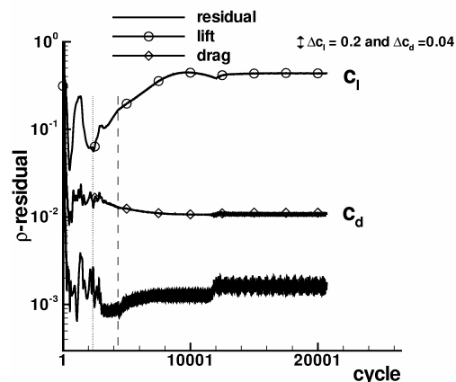
Fig. 8 Convergence history of the RANS computation, high Reynolds number take-off case, dotted: here the transition prediction process had started, long dashed: here the restart run started using fixed predicted transition locations.
