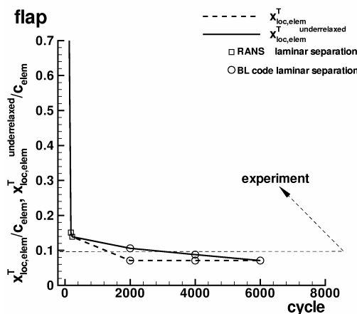
Fig. 11 Convergence histories of the transition location iteration at the slat, main airfoil and flap, low Reynolds number landing case.
