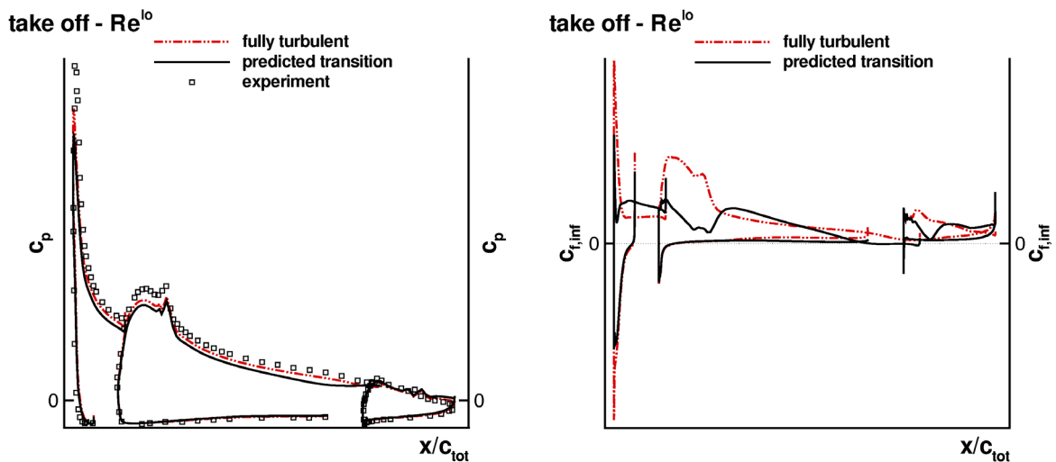
Fig. 13 c_p - and c_f -distributions, low Reynolds number take-off case, SAE turbulence model.
