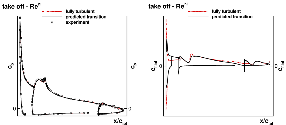
Fig. 14 c_p - and c_f -distributions, high Reynolds number take-off case, SAE turbulence model.
