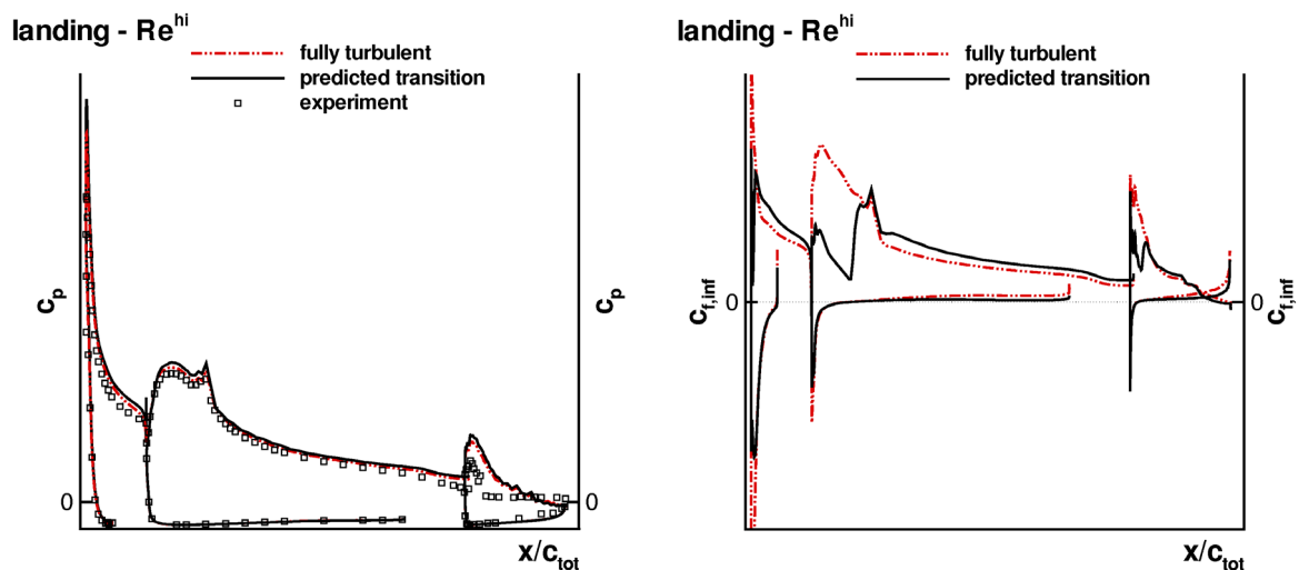
Fig. 16 c_p - and c_f -distributions, high Reynolds number landing case, Wilcox k-\omega turbulence model.
