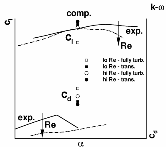
Fig. 20 Measured and computed lift coefficients, c_l , and drag coefficients, c_d , versus the angle of attack \alpha , landing case.
