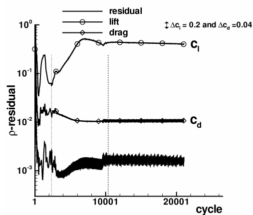
Fig. 7 Convergence history of the RANS computation, high Reynolds number take-off case, dotted: transition prediction start, dashed: transition prediction end.
