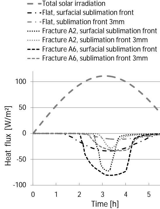
Fig. 15. Diurnal sublimation rates for a sublimation front at the surface and at a depth of 3 mm calculated for a heliocentric distance of 3.5 AU. The solar irradiation pattern for a flat surface is shown in comparison (boldface, dashed line); values are restricted to the 6.2 h in direct illumination conditions. Fractures A2 (dotted line) and A6 (dashed line) have sublimating floors. All calculations were performed for a solar plane angle of 30^\circ and sublimation originating only from the fracture bottom.
