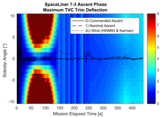
FIG 21. Maximum TVC trim deflections of the SpaceLiner Main Engines for variable sideslip angles; Non-trimmable flight conditions are hatched
