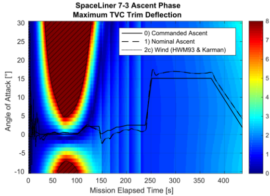
FIG 20. Maximum TVC trim deflections of the SpaceLiner Main Engines for variable angles of attack; Non-trimmable flight conditions are hatched
