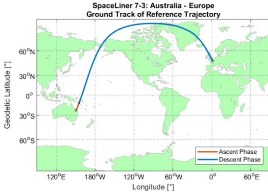
FIG 3. Ground track of the SpaceLiner reference mission from Australia to Europe
