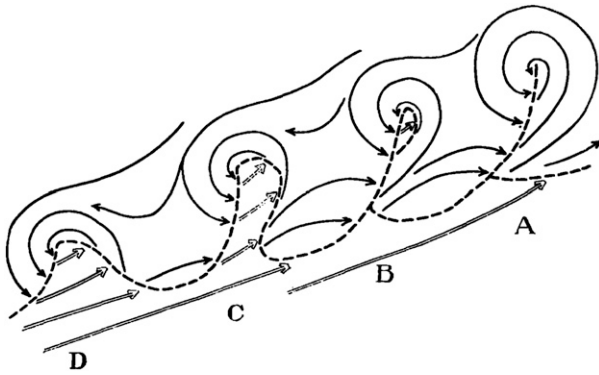
FIG. 16-8. A train of frontal-wave cyclones (Bjerknes and Solberg 1922, their Fig. 9). The figure is provided through the courtesy of the Norwegian Geophysical Society.
