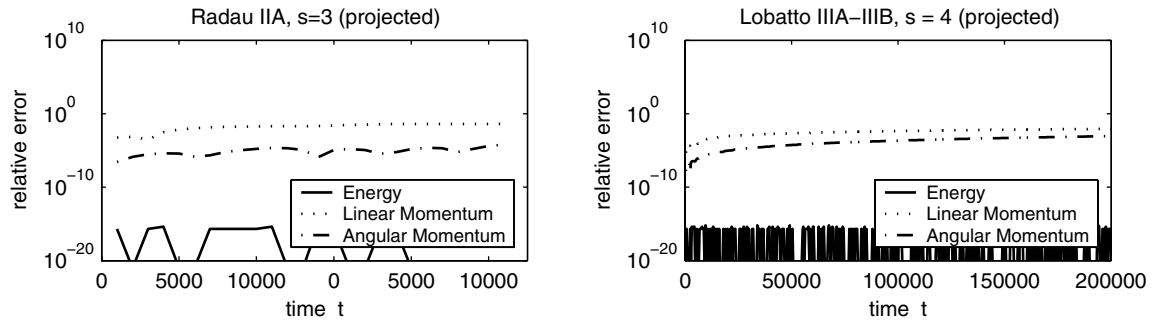
Figure 2: Errors in invariants of the 6-body problem. Classical Runge–Kutta methods with projection steps.
