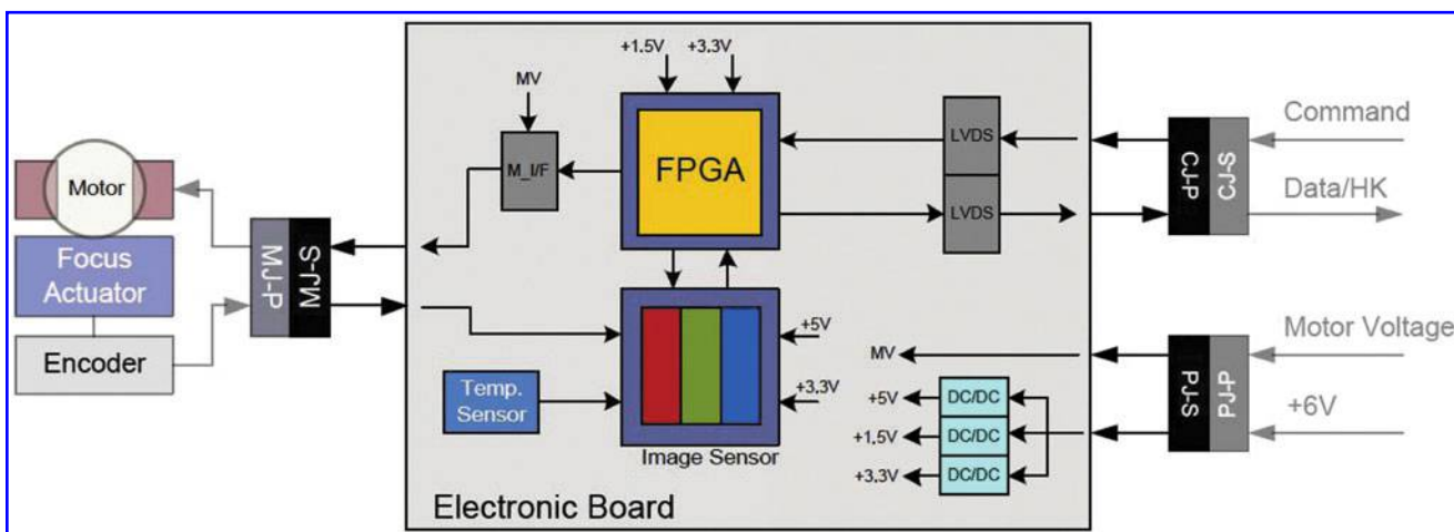
FIG. 9. HRC block diagram showing the STAR1000 CMOS sensor with temperature sensor, the FPGA (center), connectors, power conditioning, and LVDS drivers (right) and finally the focus motor control circuitry (left).
