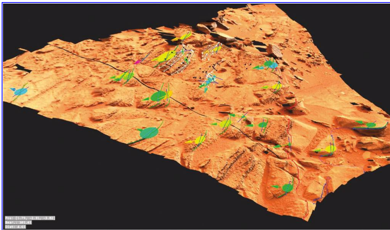
FIG. 15. Screenshot of PPro3D showing a geological interpretation session in the Shaler area (Gale Crater, MSL mission), based on PProViP 3-D reconstruction from a set of 99 MSL Mastcam stereo images. This detailed interpretation of the stratigraphy shows the main stratigraphic boundaries as gray lines, bedset boundaries as thick white lines, and laminations within those bedsets as thin white lines (note that the original image is in color). The dip and strike values are available directly in PPro3D in color coded by dip value and generally dip 15–20° to the southeast (validation forthcoming). The findings are consistent with those in the works of Anderson et al. (2015) and Edgar et al. (2014) in that the outcrop represents a changing fluvial environment, with recessive, fine-grained units interlayered with coarse, pebbly units. Data courtesy of NASA/JPL, image courtesy of Imperial College London, Robert Barnes/Sanjeev Gupta; www.provide-space.eu
