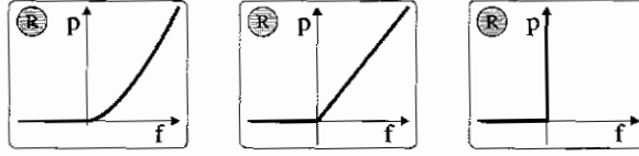
Fig. 2. Abstraction levels.
