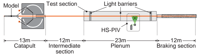
Fig. 2 Overview of the tunnel simulation facility Göttingen (cf. [6])
