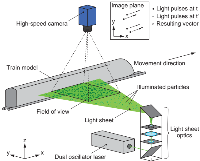
Fig. 3 Overview of the flow velocity measurement using High-Speed Particle Image Velocimetry at the tunnel simulation facility Göttingen (cf. [11])
