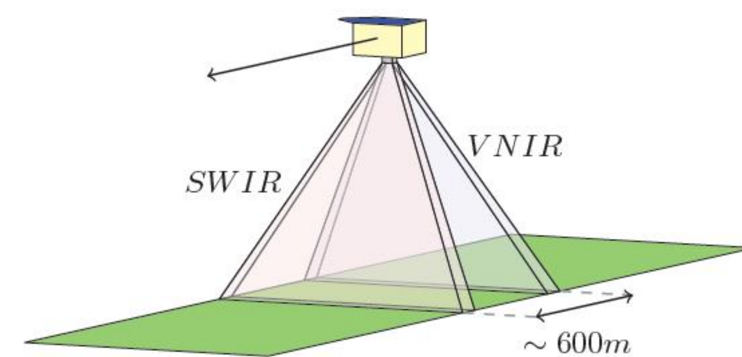
Figure illustrating the instrument design leading to a partly shift between VNIR and SWIR dataset.
