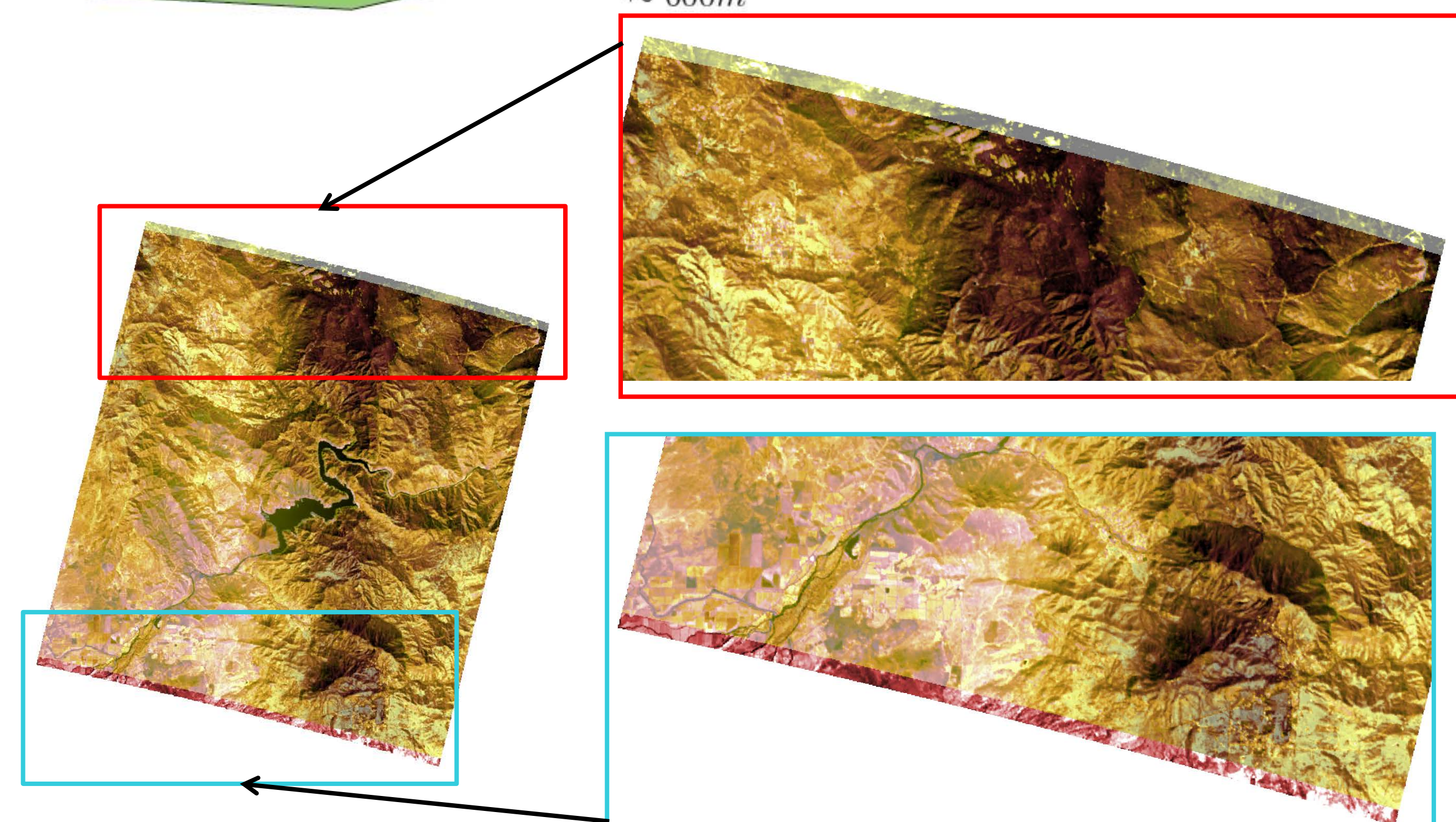
One scene, VNIR highlighted in yellow, SWIR in red. Due to instrument design the two datasets are spatially shifted in flight direction.
