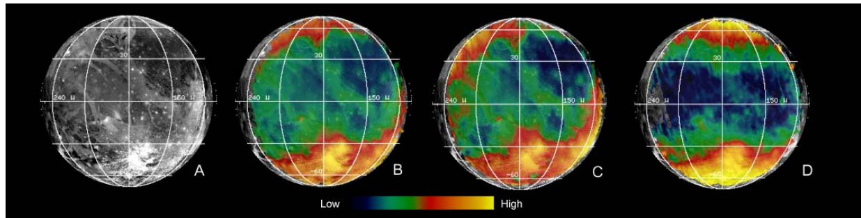
Figure 1: Comparison between visual albedo, band depths at 2 and 1.5 \mu m and ratio of band depths for the global NIMS observation of Ganymede's anti-Jovian hemisphere: (a) a global SSI image in an orthographic map projection centered at 0°lat and 180°lon compared to the measured band depths at 1.5 \mu m (b) and 2 \mu m (c), and the ratio of band depths at 2 \mu m/1.5 \mu m (d).
