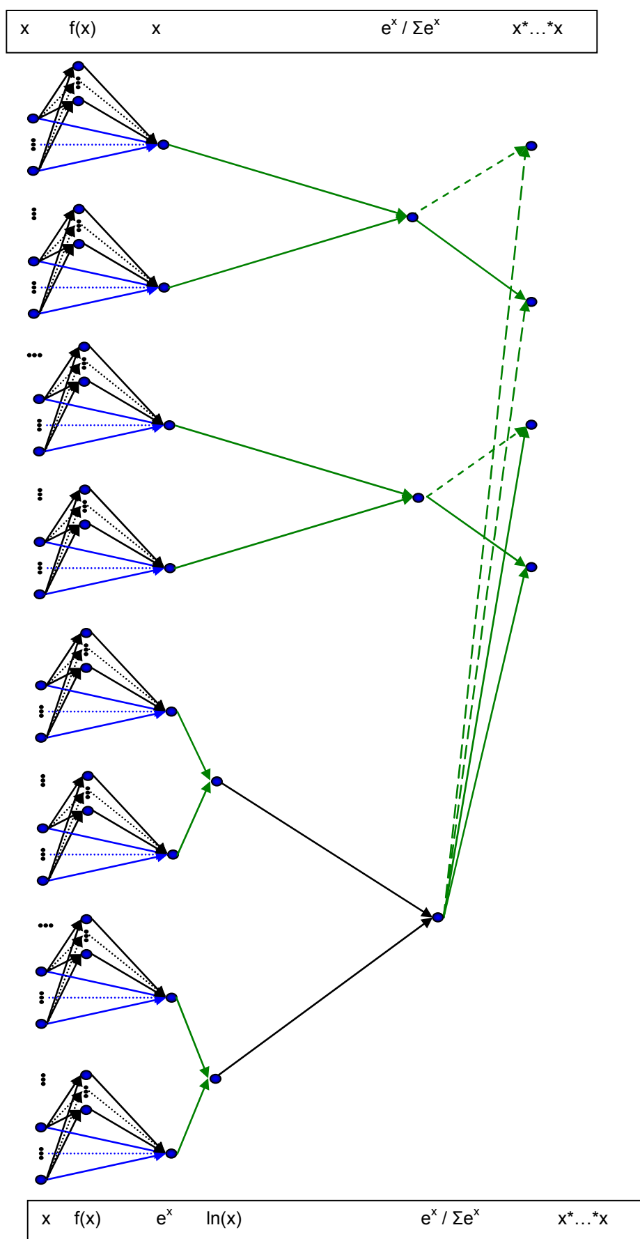
Fig. 12: Neural Nested Logit Model
